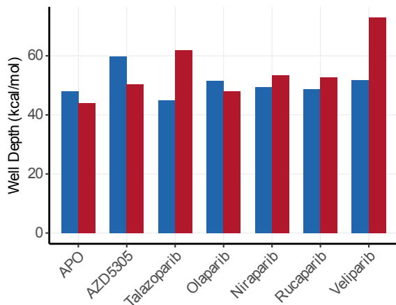
B HD-ART Energy Landscape: DNA-free vs DNA-bound
