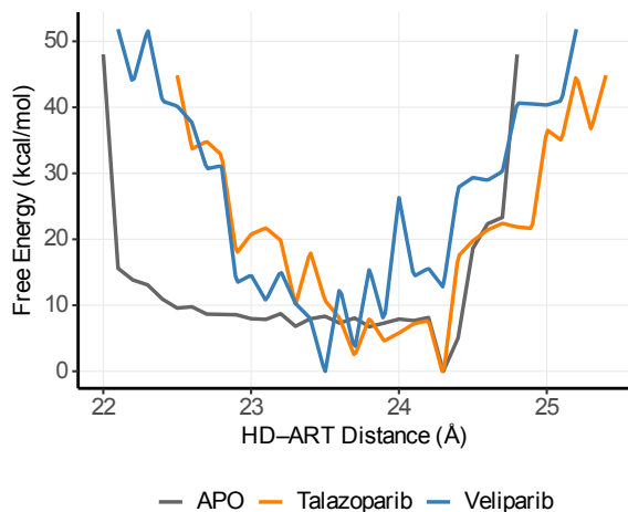
D Same CAT Pocket, Opposite Allosteric Fate
