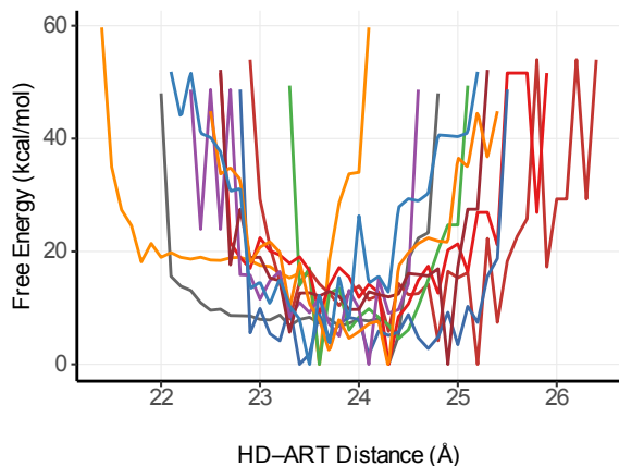
A S1: CAT-only HD-ART Free Energy Landscape
