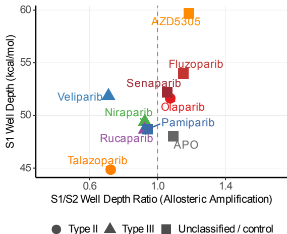
C Two-Dimensional Allosteric Mechanism Map
