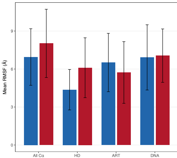
C Domain RMSF Summary
