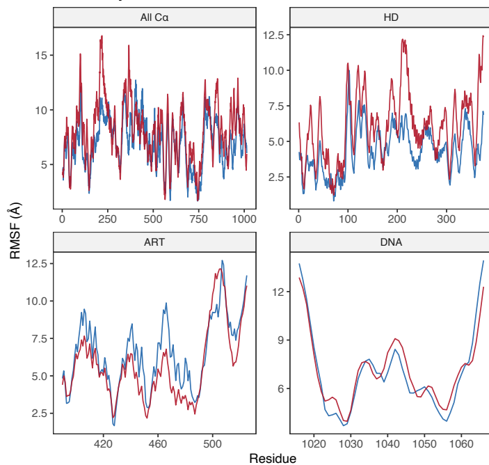
D RMSF Change upon Talazoparib Binding
