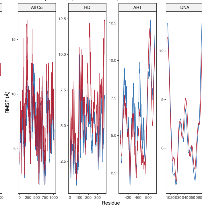
D RMSF by Residue (Full PARP1+DNA)
