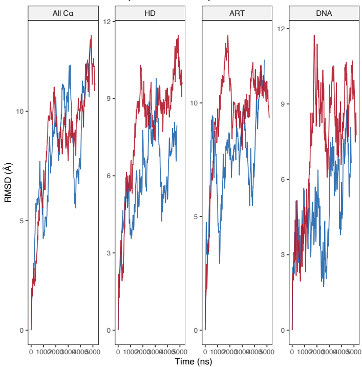
C RMSD Time Series (Full PARP1+DNA)
