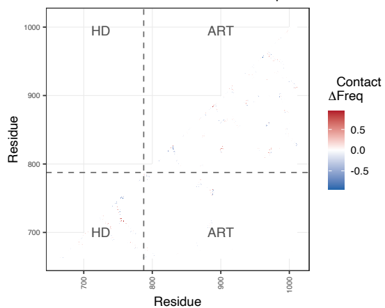
Delta Contact: AZD5305 - Veliparib
