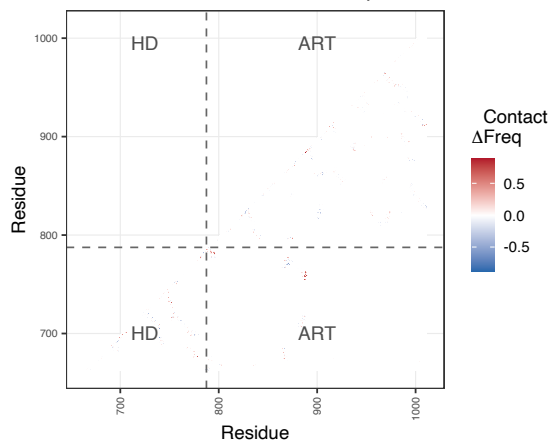
Delta Contact: Talazoparib - Veliparib
