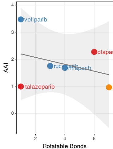
Rotatable Bonds vs AAI
