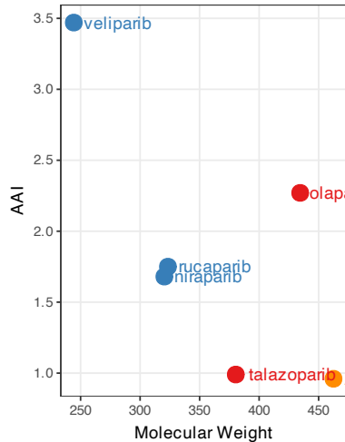
MW vs AAI
