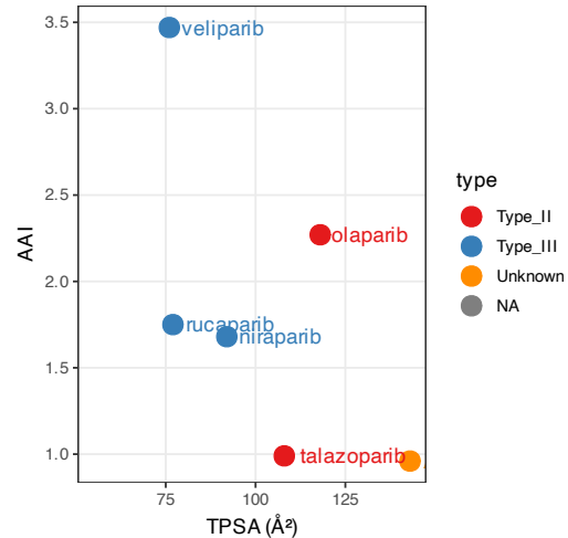
Polar Surface Area vs AAI
