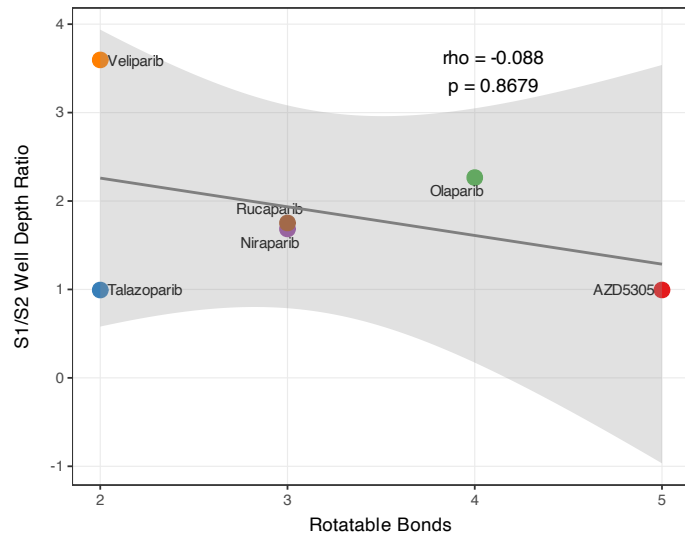
Flexibility vs DNA-Induced Stabilization
