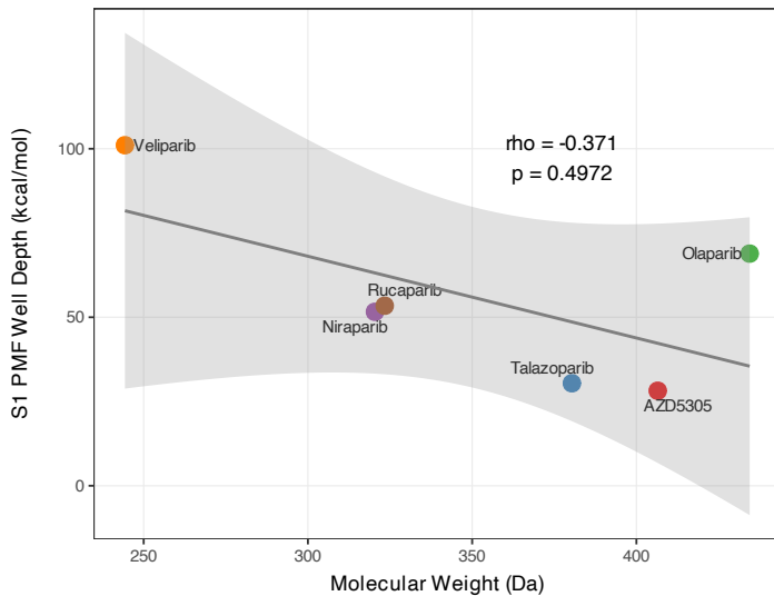
MW vs Conformational Sampling
