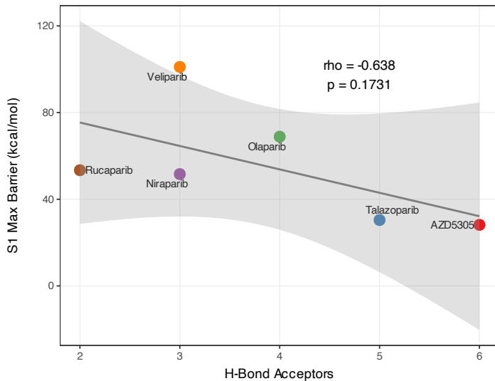
HBA Count vs Conformational Ruggedness
