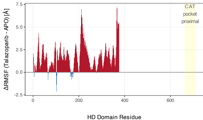
B HD Domain: Talazoparib-Induced Rigidification
