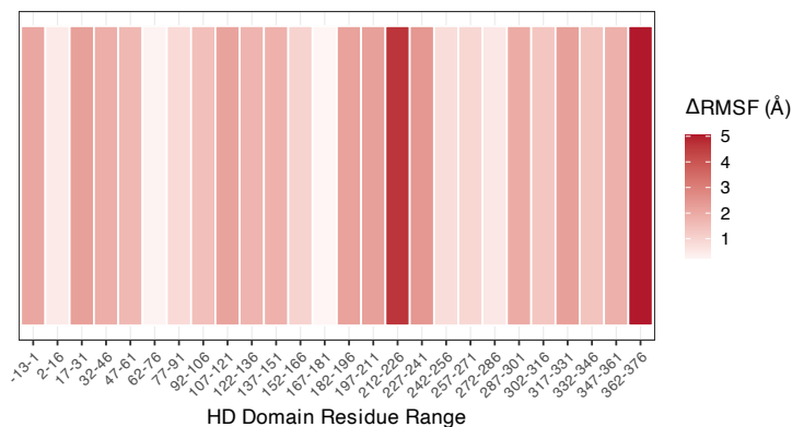
C Binned \Delta RMSF: Talazoparib Rigidifies HD Domain
