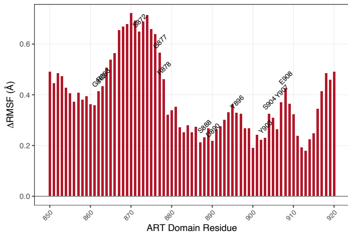
C CAT Pocket Region: Type II Rigidification
