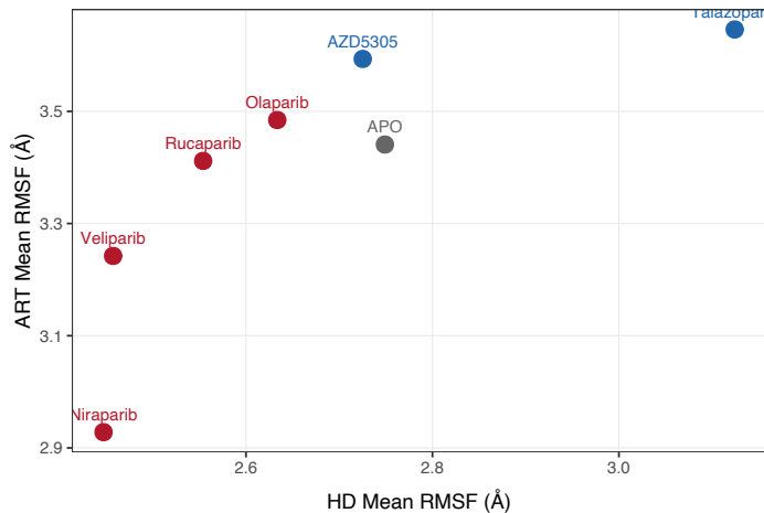
D HD vs ART Rigidity Landscape
