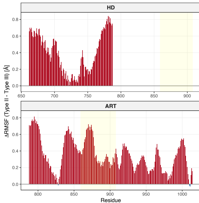
B Differential RMSF: Type II vs Type III
