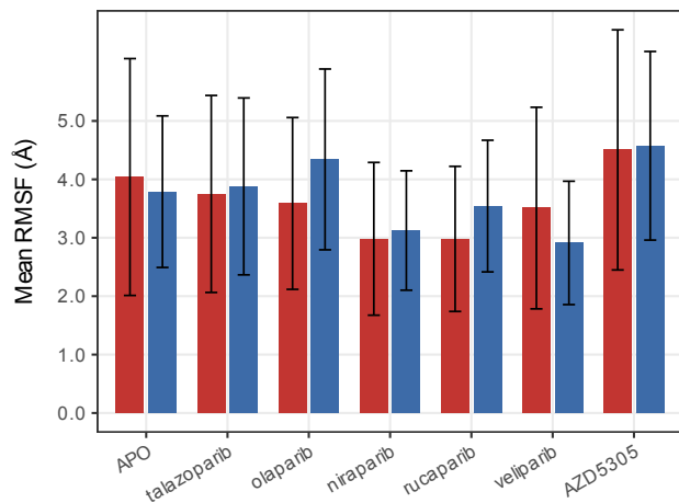
B Subdomain mean RMSF
