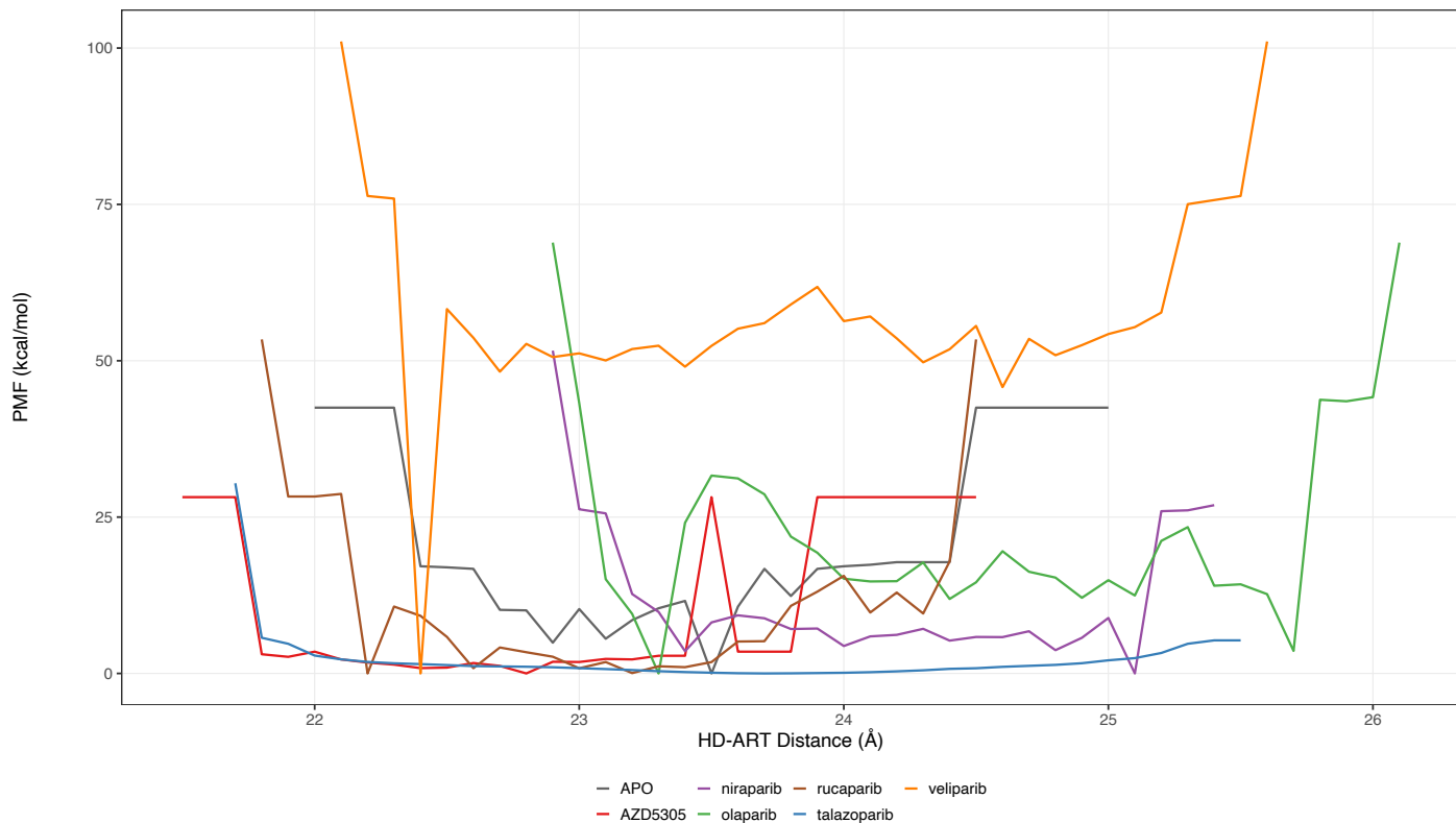
Highest Conformational Barrier by System
