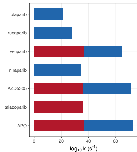
Approximate Transition Rate (Kramers)
