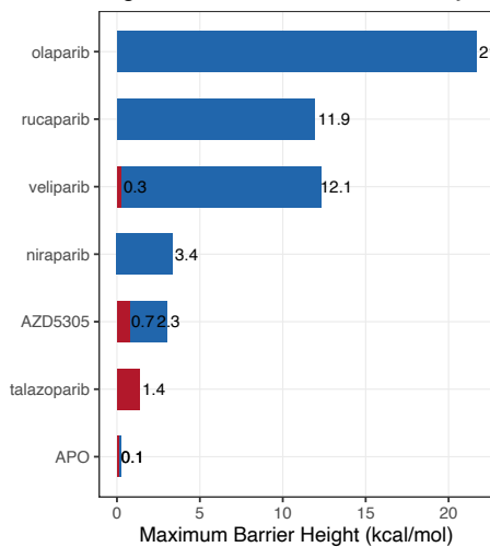
Highest Conformational Barrier by System
