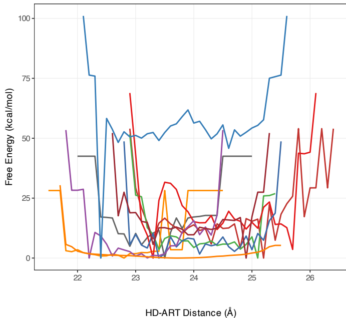
A S1: CAT-only HD-ART Free Energy Landscape
