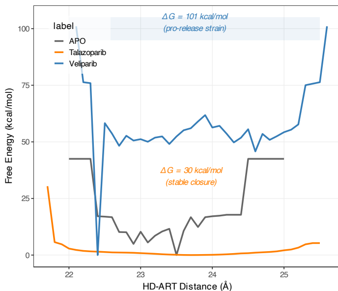
D Same CAT Pocket, Opposite Allosteric Fate
