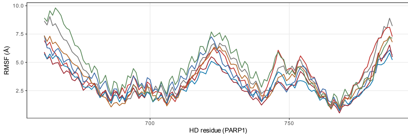
A HD per-residue RMSF
