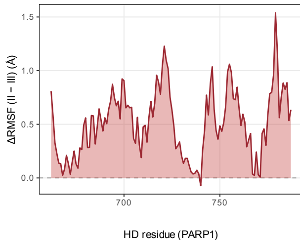
C Type II vs III \Delta RMSF
