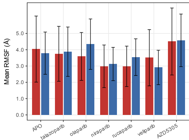
B Subdomain mean RMSF
