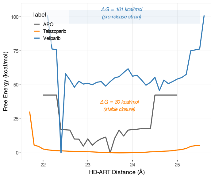
D Same CAT Pocket, Opposite Allosteric Fate
