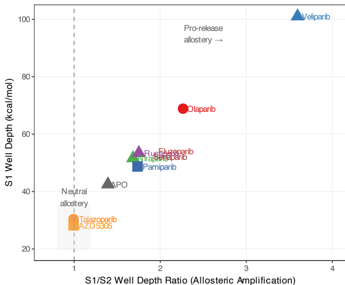
C Two-Dimensional Allosteric Mechanism Map
