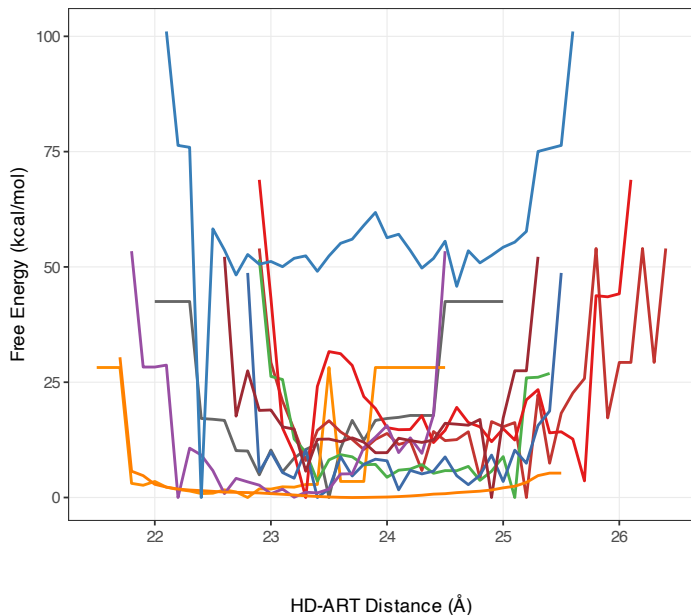
A S1: CAT-only HD-ART Free Energy Landscape
