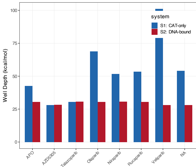
B HD-ART Energy Landscape: DNA-free vs DNA-bound
