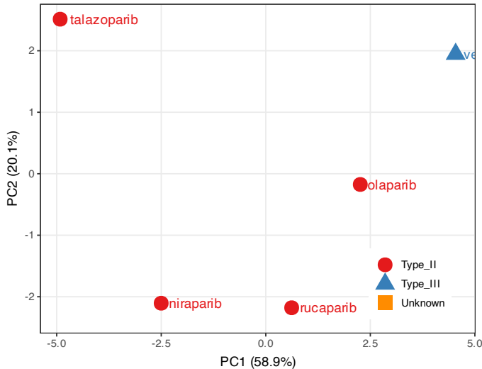
PCA: PMF Features Separate Type II vs III
