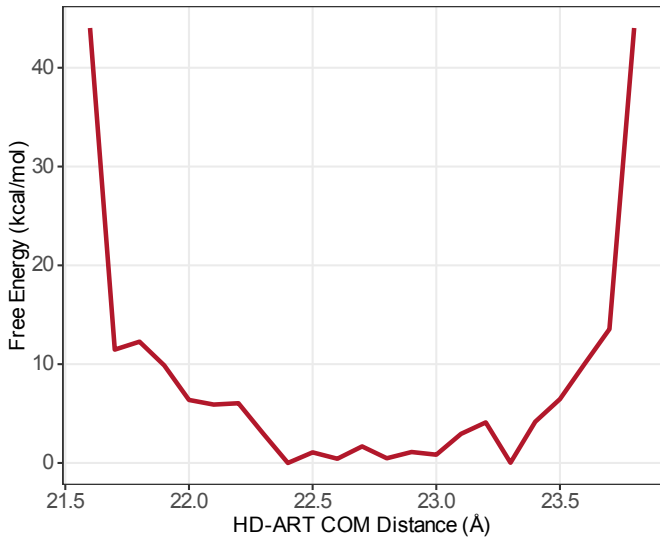
B sys2_APO — HD-ART Distance PMF
