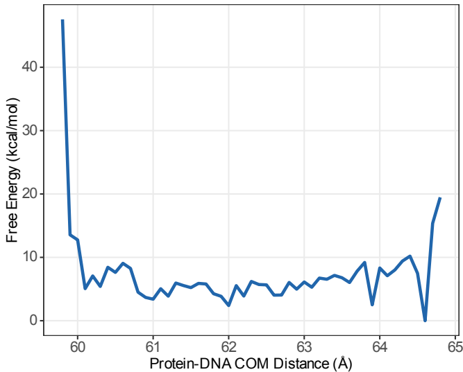
A sys2_APO — Protein-DNA Distance PMF
