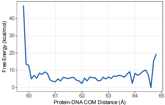
sys2_APO — Protein-DNA Distance PMF
