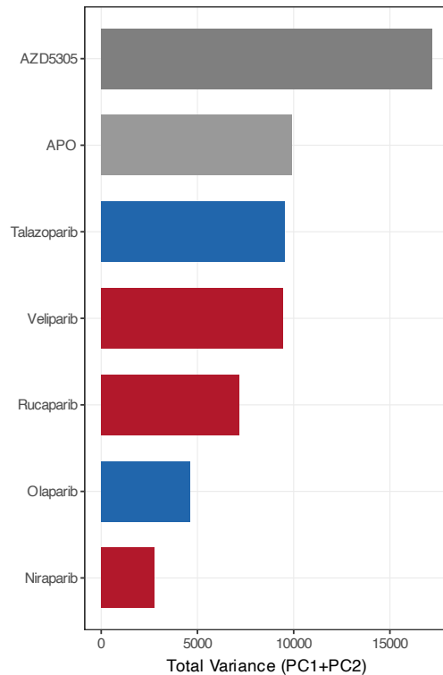
Conformational Sampling Breadth by System
