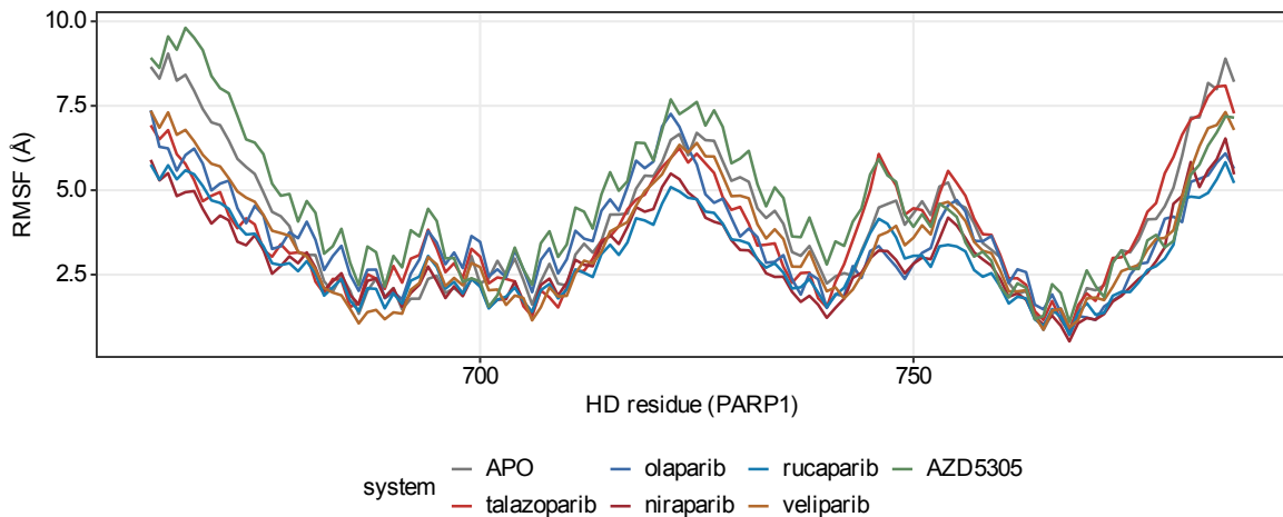
B Subdomain mean RMSF
