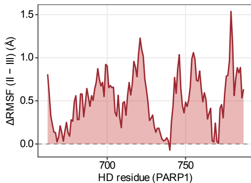
C Type II vs III \Delta RMSF
