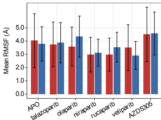
B Subdomain mean RMSF
