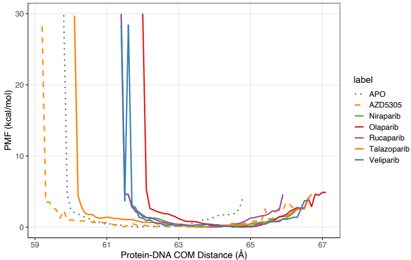
S2: PARP1-DNA Retention PMF (C3)
