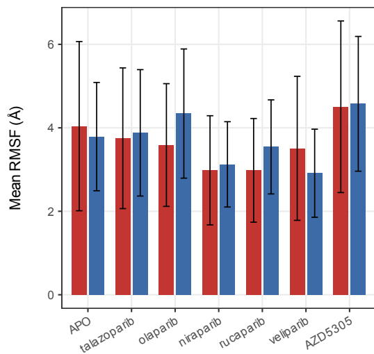
B Subdomain mean RMSF
