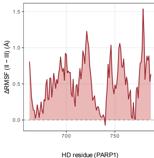
C Type II vs III \Delta RMSF
