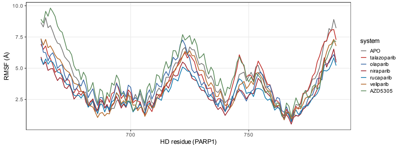
B Subdomain mean RMSF
