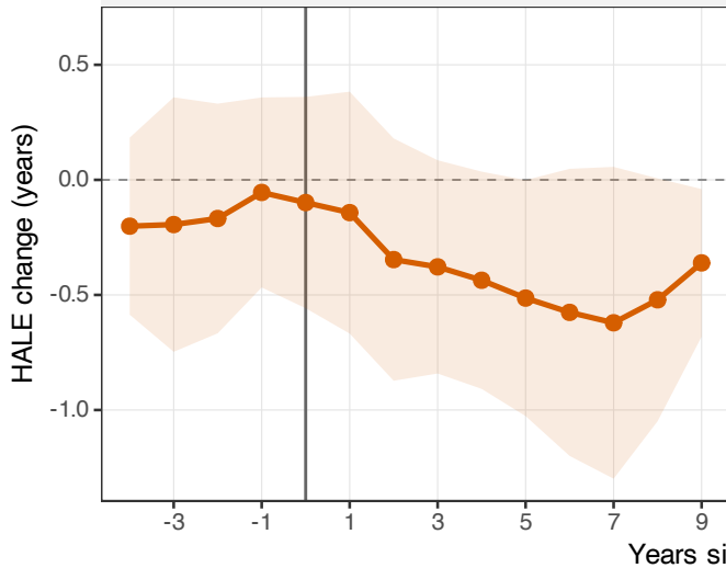
A: GHE spikes (N = 25)
