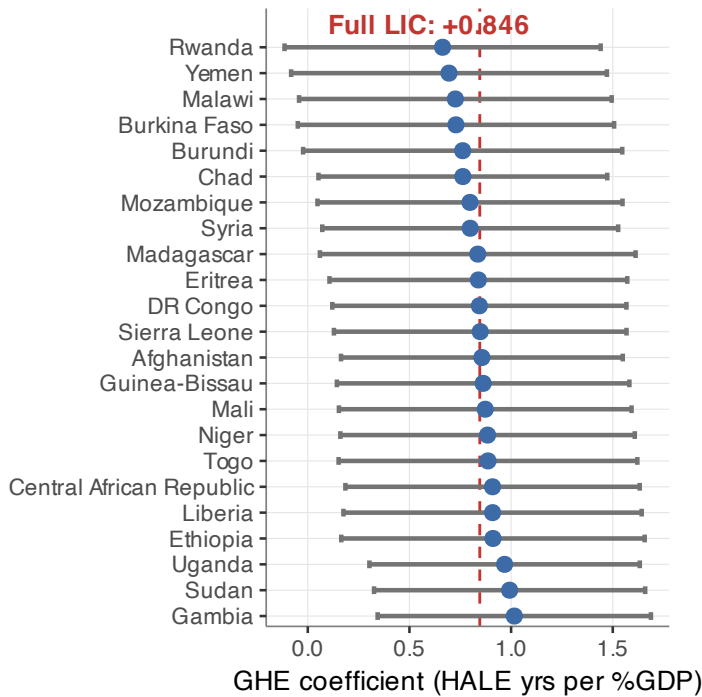
C. Lag structure (G = 23 LICs)
