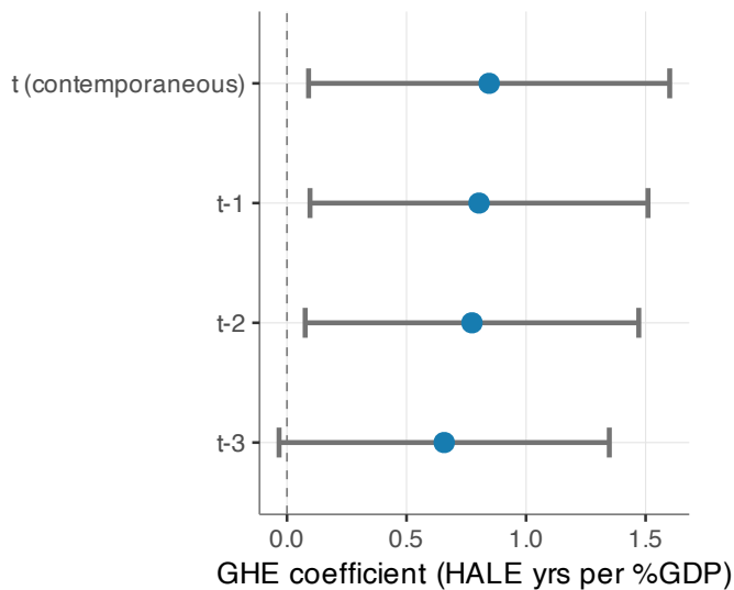
C. Lag structure (G = 23 LICs)
