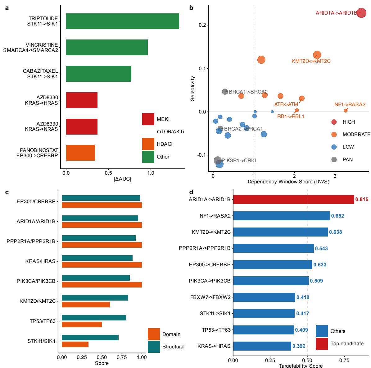
Fig. 4: Pharmacologic context and translational prioritization. a , PRISM drug selectivity: -\Delta AUC for top drug-paralog associations. Known drug-target biology is recapitulated: MEK inhibitors (AZD8330, Trametinib) selectively kill KRAS-mutant lines; mTOR/AKT inhibitors (Everolimus, Ipatasertib) kill PTEN-mutant lines; HDAC inhibitors (Panobinostat) kill EP300-mutant lines. BH q < 0.25 . See Supplementary Fig. S5 for full results. b , Therapeutic window classification. Bubble size, mean DWS; color, selectivity tier. HIGH_SELECTIVITY requires selectivity > 0.15 and DWS > 1.0 ; NF1→RASA2 has high DWS (3.26) but near-zero selectivity (0.002), hence MODERATE. c , Structural similarity (top row) and domain conservation (bottom) for 11 key paralog pairs. Filled circles, perfect domain conservation (Jaccard = 1.0). EP300↔CREBBP has the highest structural similarity (0.976). d , Composite preclinical prioritization score ranking the top 10 candidates. Scores integrate dependency window score (0.40), selectivity (0.30), structural similarity (0.15), and druggability (0.15). ARID1A→ARID1B ranks first (0.815).
