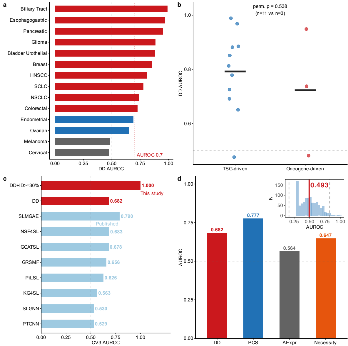
Fig. 1: Delta Dependency: pan-cancer performance, benchmark, and validation. a , DD AUROC across 14 evaluable solid tumor types (red: AUROC > 0.7; blue: 0.5–0.7; gray: < 0.5). Dashed line, random classifier (0.5). Bar labels show n tested pairs. Sample sizes and full lineage names in Supplementary Table S1. b , DD performance stratified by oncogenic mechanism. TSG-driven tumors ( n = 11 ) show numerically higher AUROC than oncogene-driven tumors ( n = 3 ; permutation p = 0.538 , not significant). Points, individual lineages; center line, group mean. c , Contextual comparison: DD AUROC vs. published CV3 values from eight deep learning methods [13]. Red bars, this study; blue bars, published values. Note: different test sets; not a head-to-head benchmark. The interpretable composite score (AUROC = 0.841) exceeds all four multi-feature classifiers tested under leave-one-pair-out cross-validation (0.138–0.744), and each DD-based nomination traces to a single measurable quantity ( |DD| ), enabling direct experimental design, whereas multi-feature classifiers produce opaque scores. d , Component decomposition: DD (AUROC = 0.682) versus PCS (0.777), \Delta Expression alone (0.564), and necessity (0.647). Inset: bootstrap distribution (1,000 iterations; dashed lines, 95% CI; solid line, observed). Full bootstrap and negative control in Supplementary Fig. S8.
