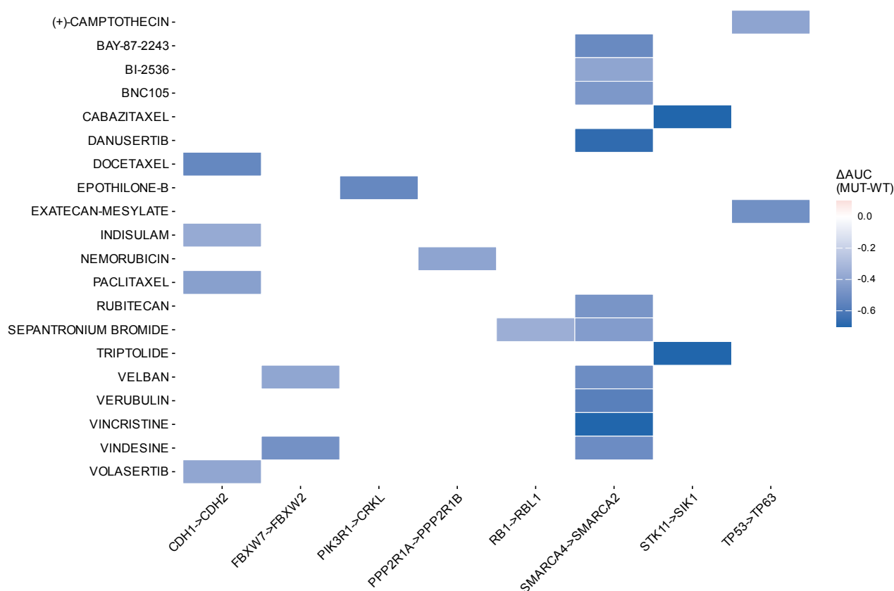
Fig. S5: PRISM drug selectivity heatmap. Heatmap of drug sensitivity differential ( \Delta\text{AUC} = mean AUC in driver-mutant minus mean AUC in wild-type cell lines) for the top driver-genotype–drug sensitivity associations from the PRISM Repurposing screen (1,482 compounds, 727 cell lines). Negative \Delta\text{AUC} indicates selective sensitivity in driver-mutant cells. Associations shown met discovery-stage criteria (BH q < 0.25 , \Delta\text{AUC} < 0 , enrichment > 0.1 ). Known drug–target biology is recovered: MEK inhibitors with KRAS-mutant lines, mTOR/AKT inhibitors with PTEN-mutant lines, HDAC inhibitors with EP300-mutant lines. Drugs shown are not necessarily direct binders of the paralog protein.
