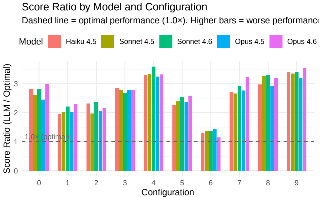
Figure 3: Score Ratio (LLM / Optimal) by Model and Configuration
