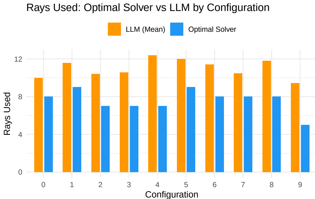
Figure 1: Rays Used: LLM (mean across conditions) vs Optimal Solver by Configuration
