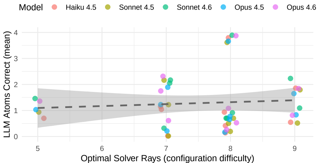
Figure 4: Configuration Difficulty (Optimal Rays) vs LLM Atoms Correct
