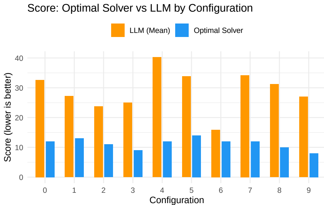
Figure 2: Score: LLM (mean across conditions) vs Optimal Solver by Configuration
