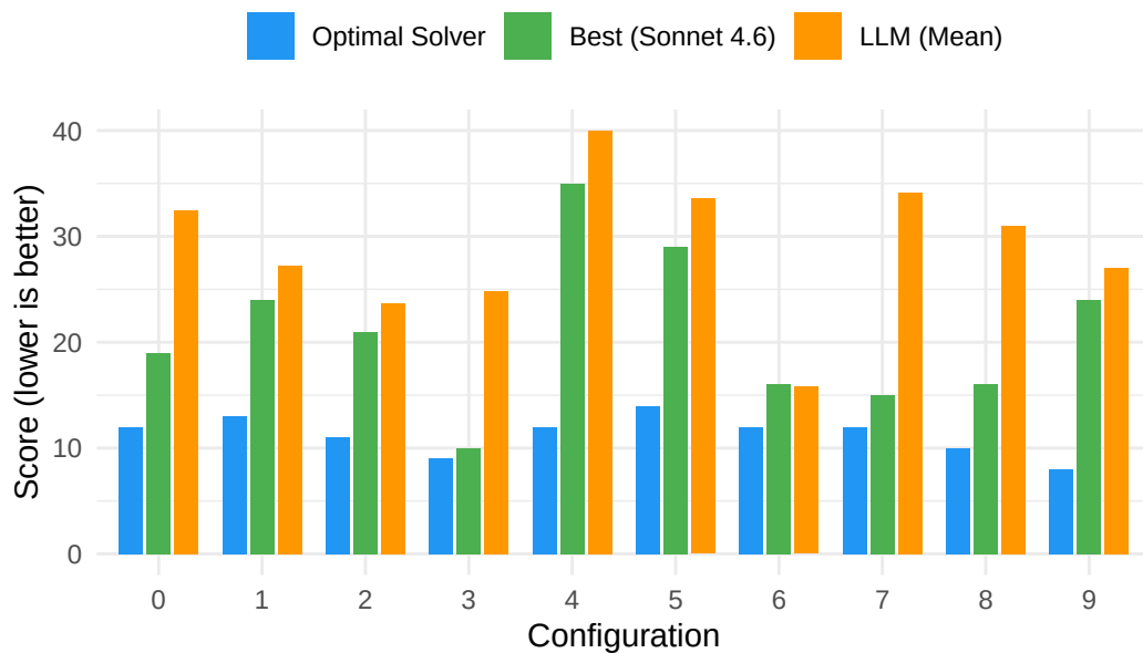
Figure 2: Score: LLM (mean across conditions) vs Optimal Solver by Configuration
