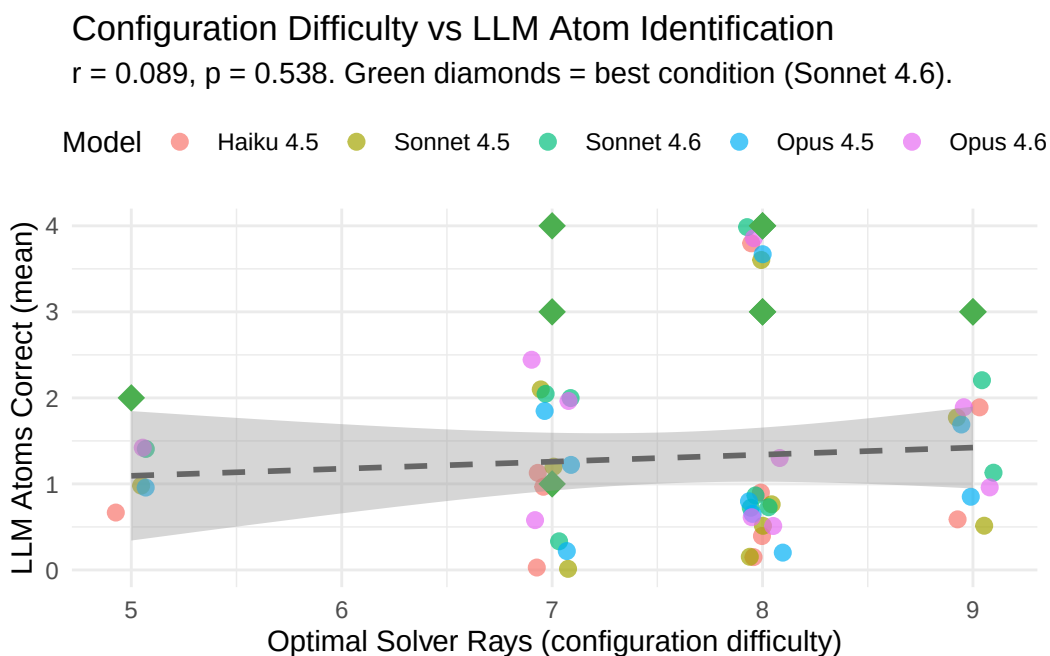
Figure 4: Configuration Difficulty (Optimal Rays) vs LLM Atoms Correct
