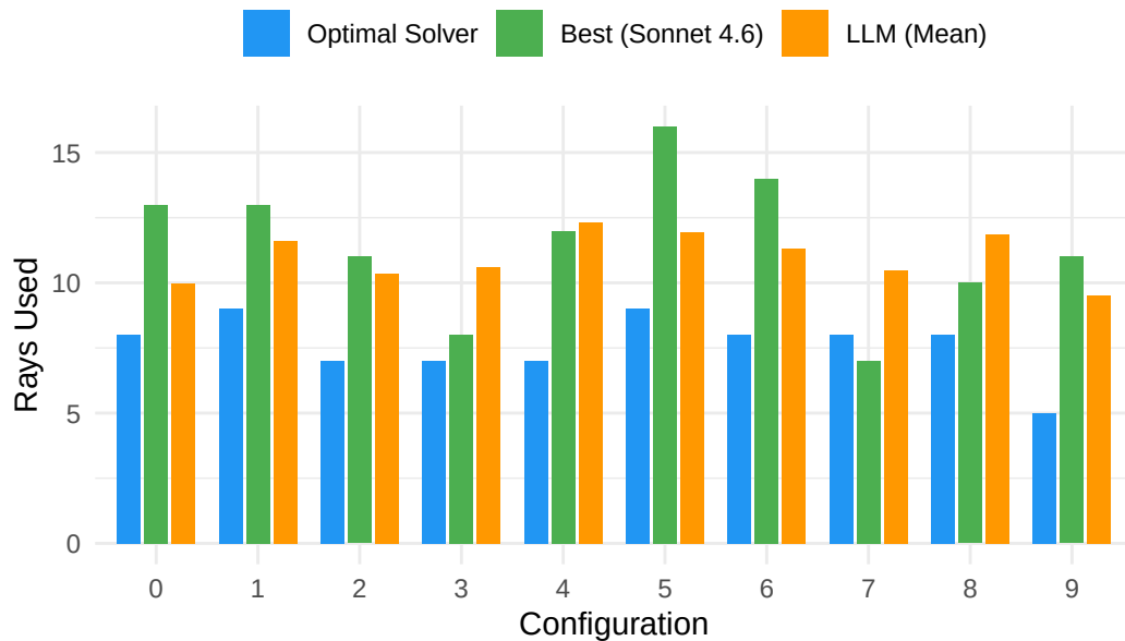
Figure 1: Rays Used: LLM (mean across conditions) vs Optimal Solver by Configuration
