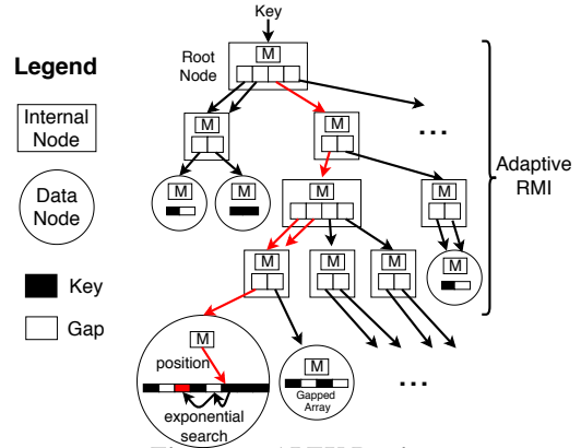
Figure 2: ALEX Design
