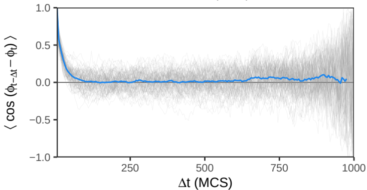
directional autocorrelation (DAC)
