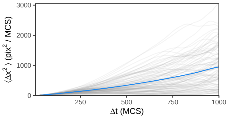
mean squared displacement (MSD)
