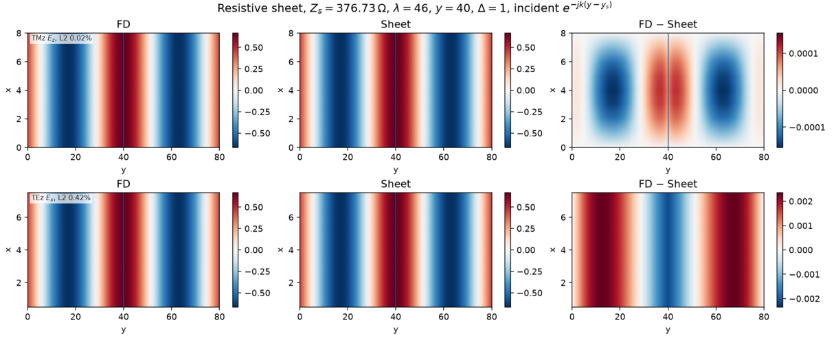
Figure 15: Resistive sheet at Z_s = \eta_0 , \lambda = 46 , y = 40 , on an 8 \times 80 box at \Delta = 1 . The rows are \text{Re } E_z (TMz) and \text{Re } E_x (TEz). The annotated L^2 is the packed free electric vector.
