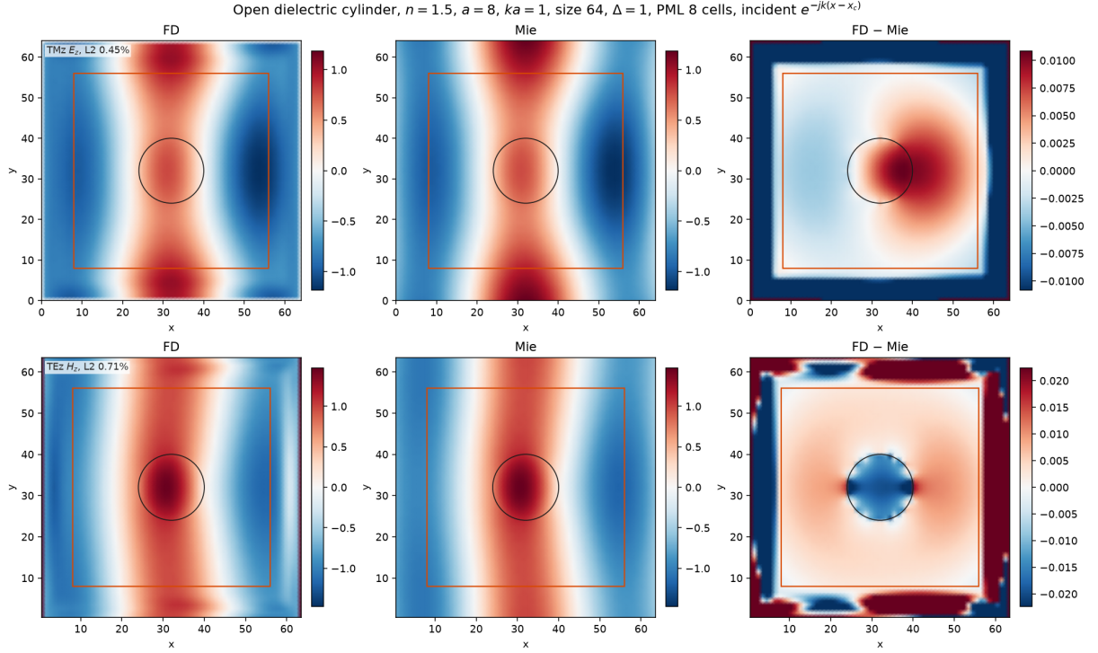
Figure 10: Open dielectric cylinder at n = 1.5 , ka = 1 , a = 8 , \Delta = 1 , with eight PML cells on each side. The annotated L^2 errors are the electric samples in the unstretched window, at least 2\Delta off the circle.
