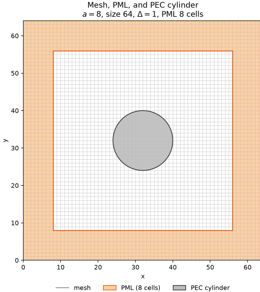
Figure 7: Default open-cylinder domain. The orange frame is the PML band used by the solve. The disk is the staircase PEC.
