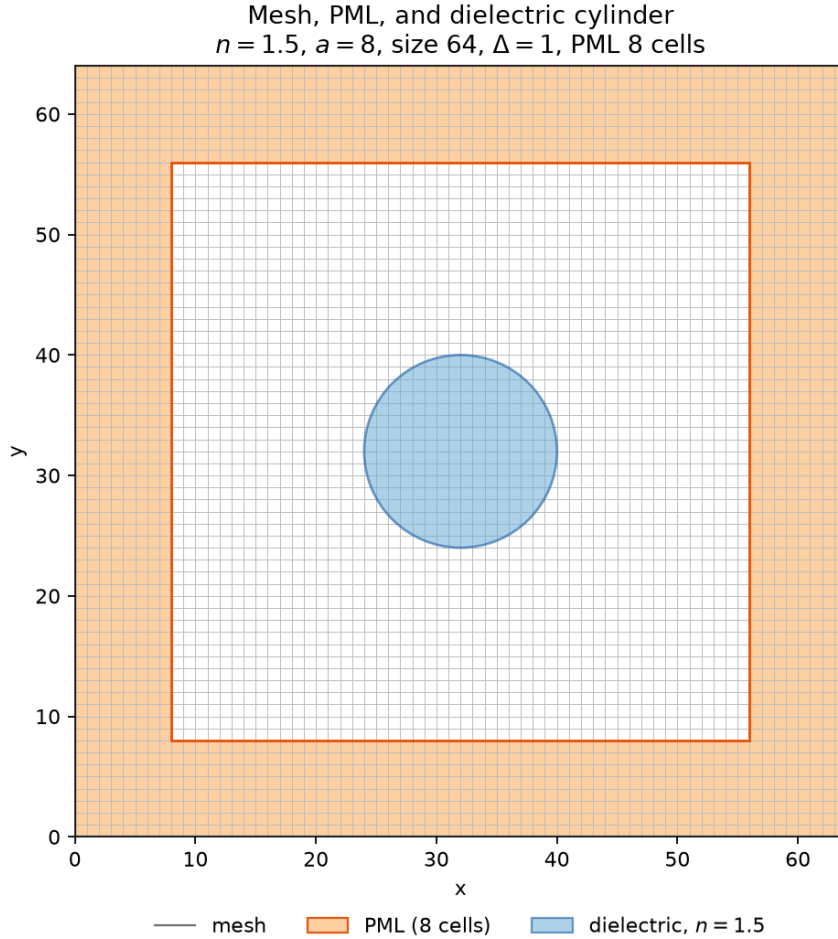
Figure 9: Default open dielectric domain. The orange frame is the PML band used by the solve. The disk is the staircase dielectric, n = 1.5 .
