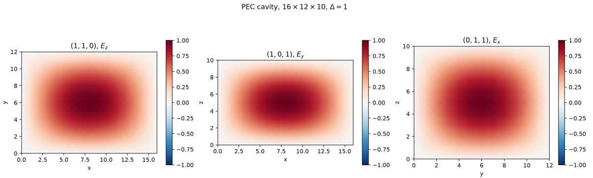
Figure 11: Pure modes of a 16 \times 12 \times 10 PEC cavity at \Delta = 1 . (1, 1, 0) is E_z(x, y) , (1, 0, 1) is E_y(x, z) , and (0, 1, 1) is E_x(y, z) .
