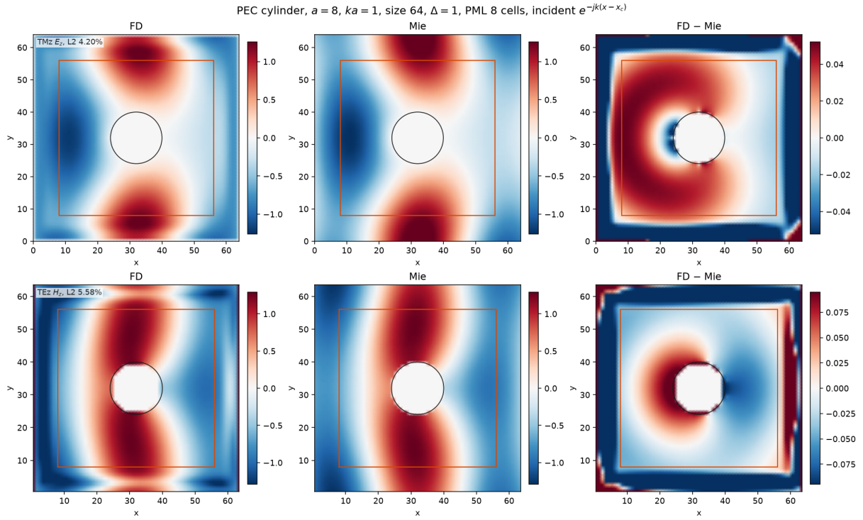
Figure 8: Open PEC cylinder at ka = 1 , a = 8 , \Delta = 1 , with eight PML cells on each side. The annotated L^2 errors are the electric samples in the unstretched window, at least 2\Delta outside the circle.
