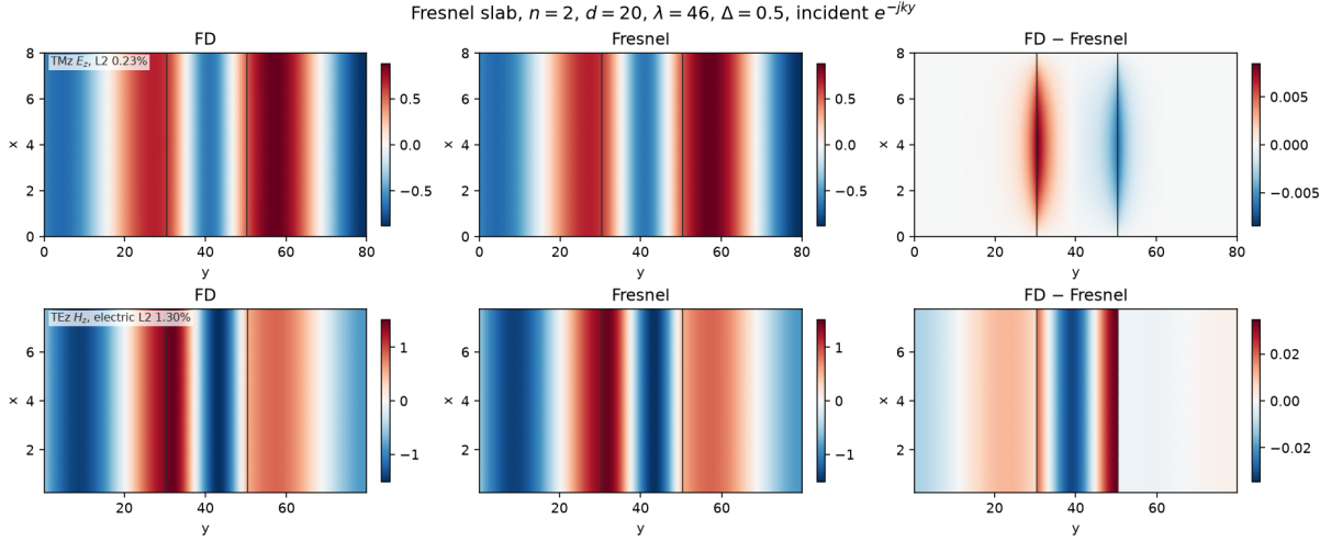
Figure 3: Default Fresnel maps. Vertical lines mark the slab faces. H_z is rebuilt with (10). The annotated L^2 errors are the free electric samples.
