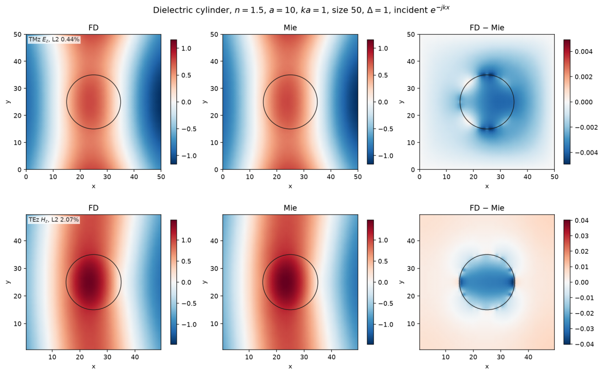
Figure 5: Default cylinder maps against the Mie series at ka = 1 , n = 1.5 .
