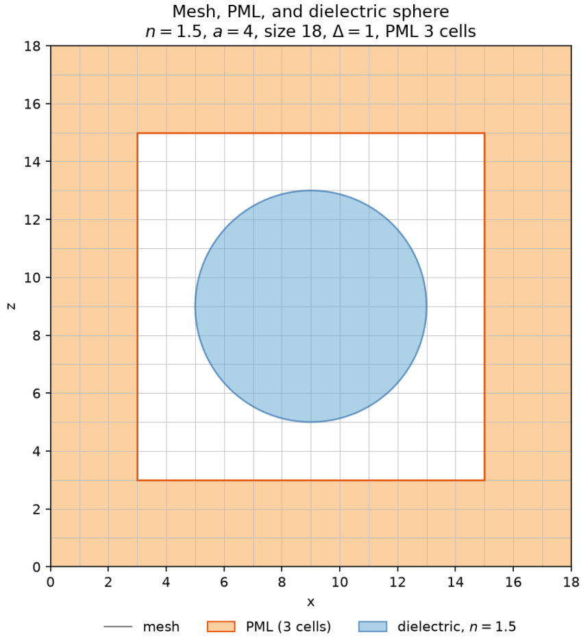
Figure 12: Default open-sphere domain. The orange frame is the PML band used by the solve. The disk is the cross-section of the staircase ball, n = 1.5 .
