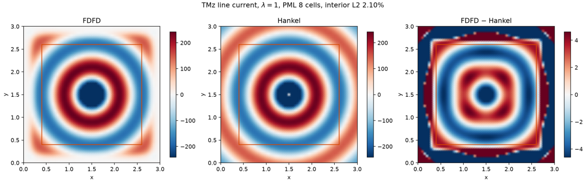
Figure 6: Line current at \lambda = 1 on a 3 m box, \Delta = 0.05 m, with eight PML cells on each side. The orange square is the inner edge of the band. The annotated error is the interior window described above.
