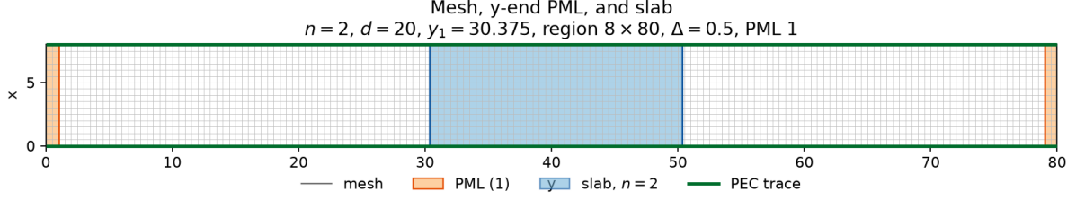
Figure 2: Default Fresnel domain. Orange bands are the y -end PML thickness drawn on the figure. Green edges are the PEC trace at x = 0 and x = 8 .
