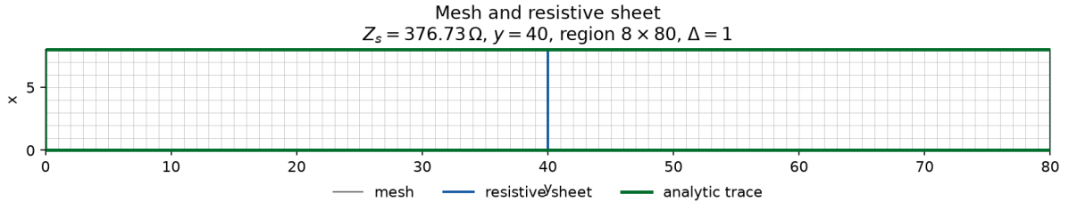
Figure 14: Default resistive-sheet domain. The blue line is the sheet. The green frame is the analytic trace on all four walls.
