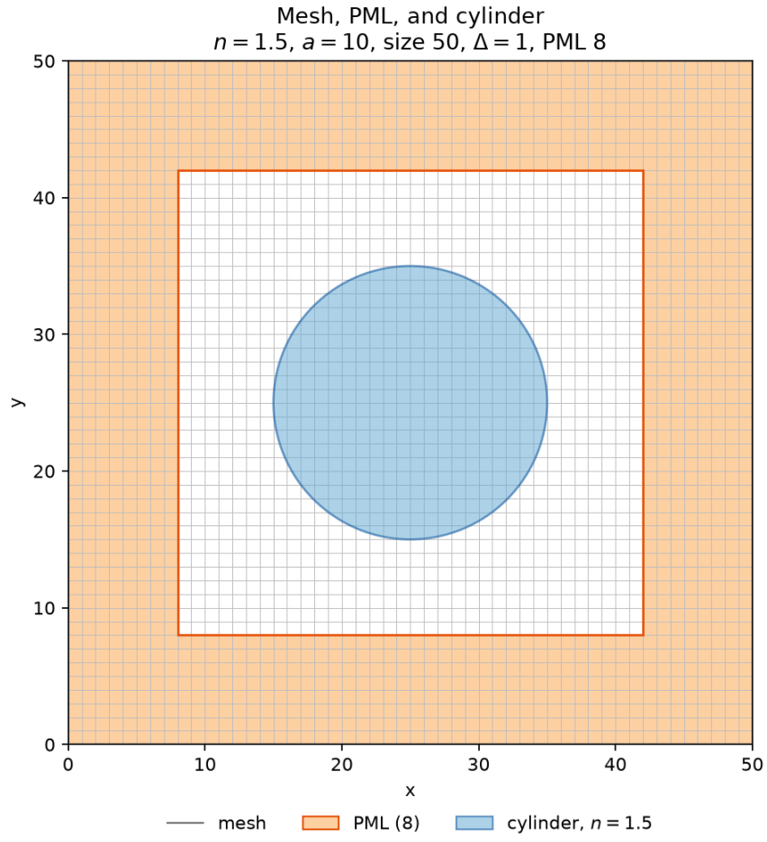
Figure 4: Default cylinder domain. The orange frame is the drawn PML thickness. The disk is the staircase geometry. The outer boundary of the solve remains the PEC trace.
