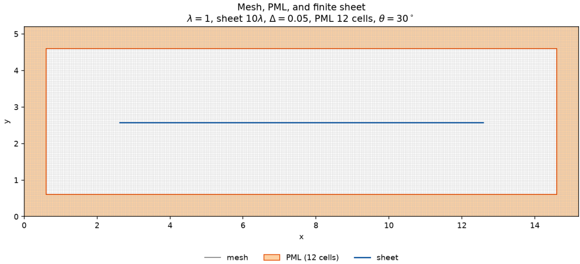
Figure 28: Finite magneto-electric domain. The blue segment is the 10\lambda sheet on a magnetic face. The orange frame is the PML band on all four sides. The incidence is 30^\circ and the susceptibilities add \chi_{em} = \chi_{me} = 0.2 to the values of Figure 24.
