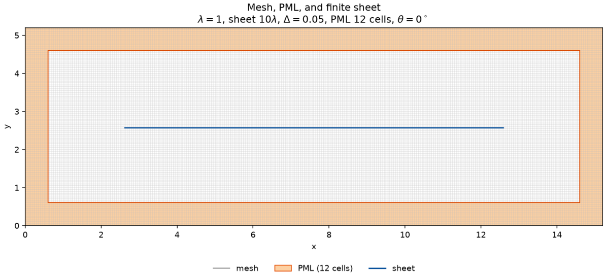
Figure 25: Default finite-sheet domain. The blue segment is the 10\lambda sheet on a magnetic face. The orange frame is the PML band on all four sides. The wall behind that band is PEC.
