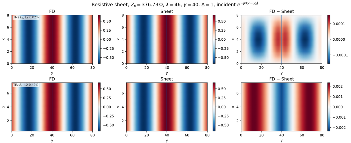
Figure 22: Resistive sheet at Z_s = \eta_0 , \lambda = 46 , y = 40 , on an 8 \times 80 box at \Delta = 1 . The rows are \text{Re } E_z (TMz) and \text{Re } E_x (TEz). The annotated L^2 is the packed free electric vector.
