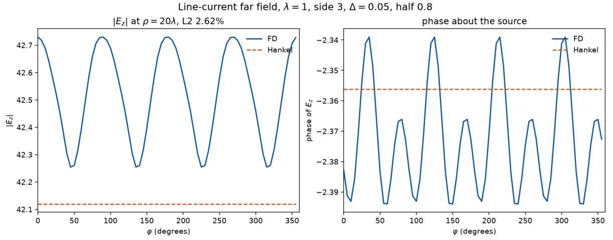
Figure 20: Line-current far field at \lambda = 1 , on a square of side 3 at \Delta = 0.05 , with eight PML cells on each face and a contour of half-width 0.8. The panels are |E_z| and the phase at \rho = 20\lambda . The annotated L^2 is the complex error against the leading Hankel wave.
