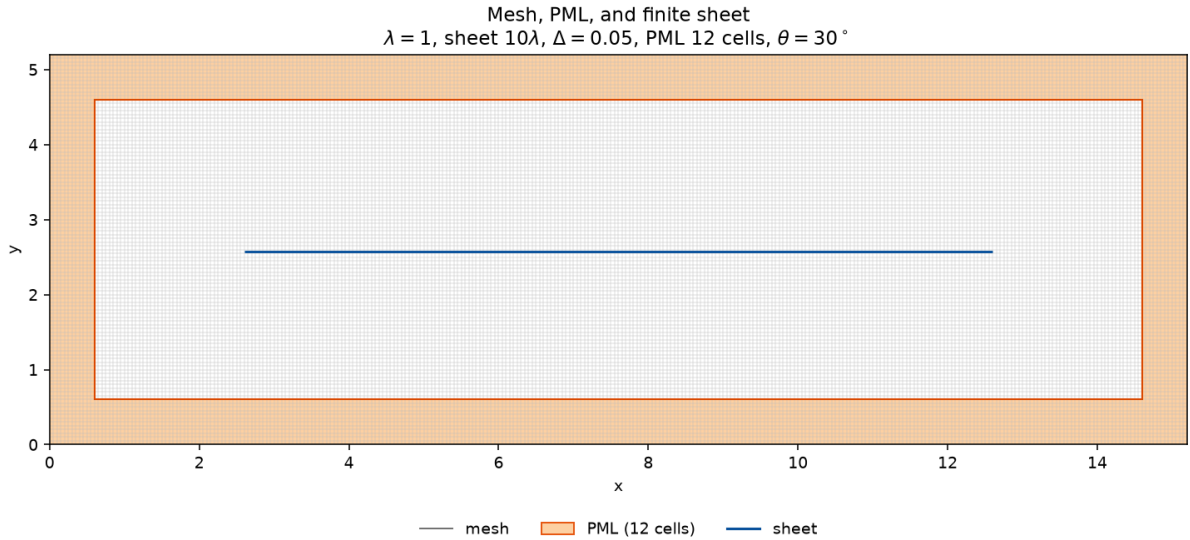
Figure 30: Finite oblique-sheet domain. The blue segment is the 10\lambda sheet on a magnetic face. The orange frame is the PML band on all four sides. The incidence is 30^\circ and the susceptibilities are \chi_{ee} = 0.5 , \chi_{mm} = 0.25 , \chi_{mm}^{nn} = 0.4 .
