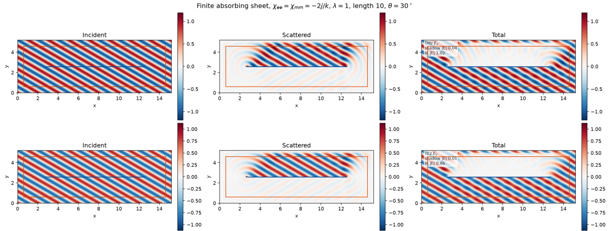
Figure 27: Finite absorbing sheet at \theta = 30^\circ , with \chi_{ee} = \chi_{mm} = -2j/k , \lambda = 1 , and length 10\lambda . The rows are \text{Re } E_z (TMz) and \text{Re } E_x (TEz). The annotated means are the lit side and the shadow over the central 6\lambda of the sheet.
