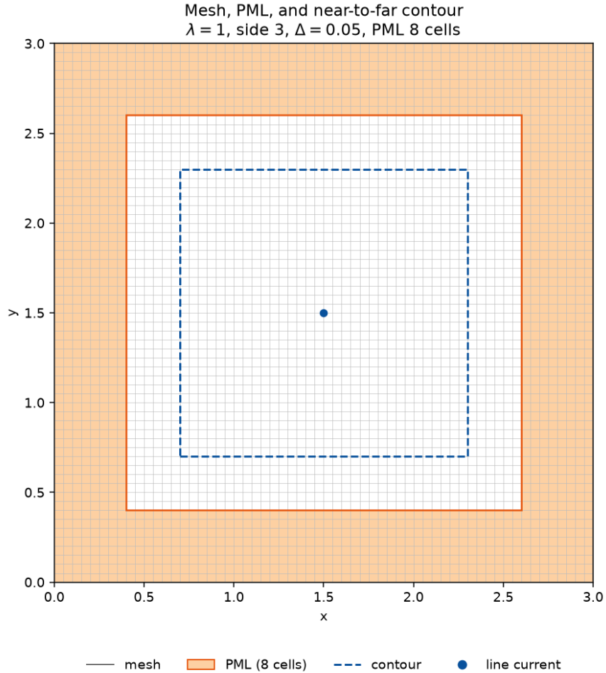
Figure 19: Default line-current far-field domain. The orange frame is the PML band used by the solve. The dashed square is the near-to-far contour. The blue dot is the line current.
