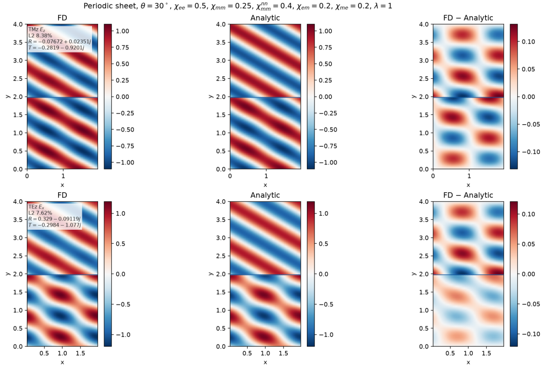
Figure 33: Periodic oblique sheet at \chi_{ee} = 0.5 , \chi_{mm} = 0.25 , \chi_{mm}^{nn} = 0.4 , \chi_{em} = \chi_{me} = 0.2 , \lambda = 1 , \theta = 30^\circ , and a height of 4\lambda , on a 40 \times 80 grid at \Delta = 0.05 . The rows are \text{Re } E_z (TMz) and \text{Re } E_x (TEz). The columns are the Yee field, the analytic field, and their difference. The annotated L^2 is the packed free electric vector.
