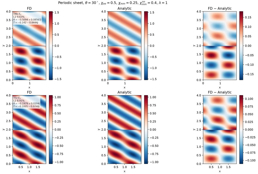
Figure 29: Periodic oblique sheet at \chi_{ee} = 0.5 , \chi_{mm} = 0.25 , \chi_{mm}^{nn} = 0.4 , \lambda = 1 , \theta = 30^\circ , and a height of 4\lambda , on a 40 \times 80 grid at \Delta = 0.05 . The rows are \text{Re } E_z (TMz) and \text{Re } E_x (TEz). The columns are the Yee field, the analytic field, and their difference. The annotated L^2 is the packed free electric vector.
