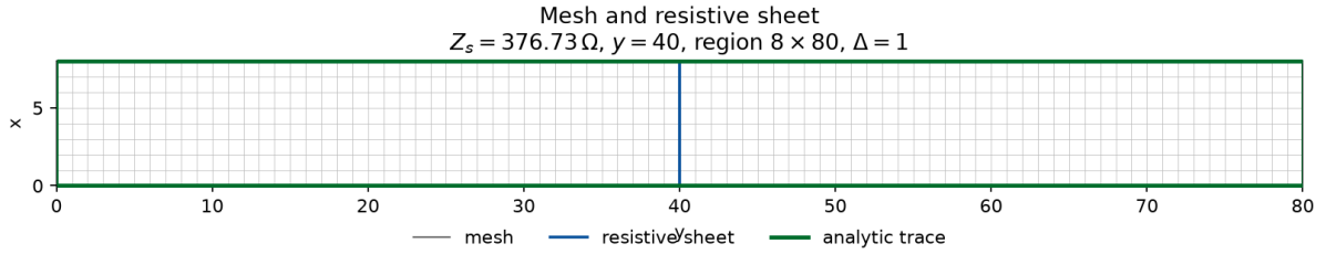
Figure 19: Default resistive-sheet domain. The blue line is the sheet. The green frame is the analytic trace on all four walls.
