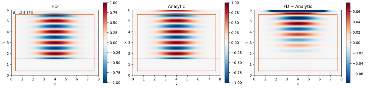
Gaussian beam, w_0 = 1.5 , \lambda = 1 , 8 \times 6 , \Delta = 0.05 , PML 8 cells
