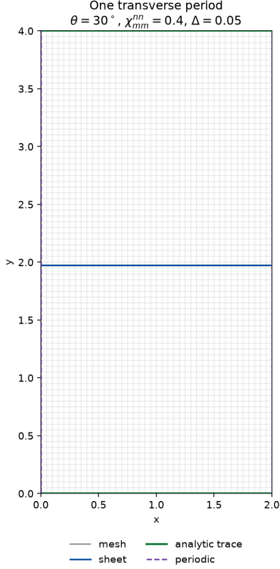
Figure 26: Default periodic-sheet domain. The blue line is the sheet on a magnetic face. The green lines are the analytic trace on the y ends. The dashed purple lines mark the periodic identification of the x ends. The width is one transverse period at 30^\circ .
