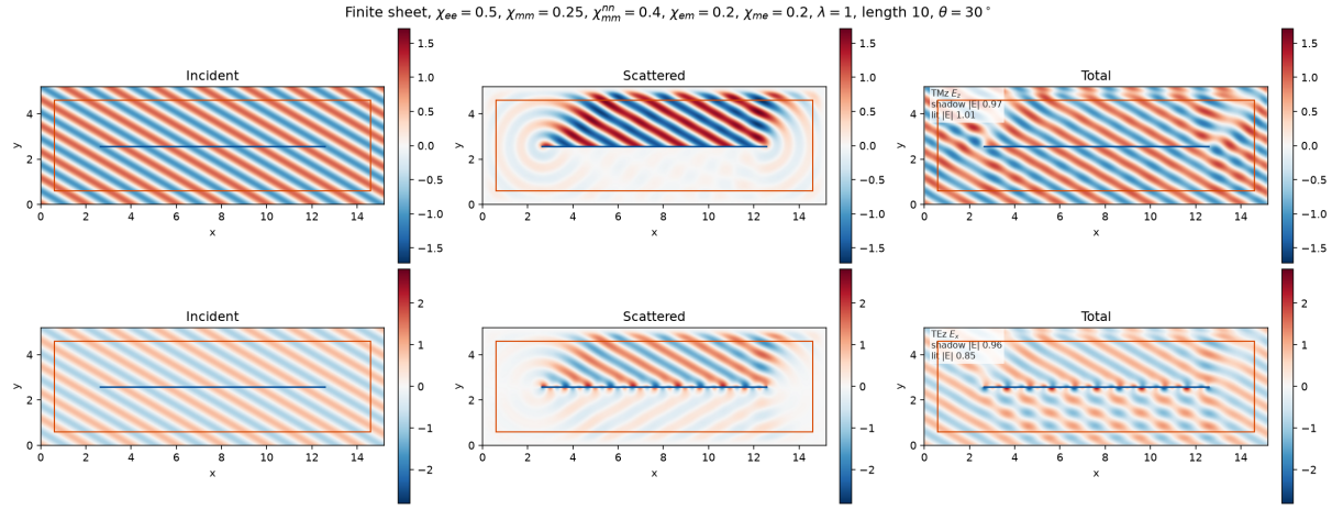
Figure 33: Finite sheet at \chi_{ee} = 0.5 , \chi_{mm} = 0.25 , \chi_{mm}^{nn} = 0.4 , \chi_{em} = \chi_{me} = 0.2 , \lambda = 1 , length 10\lambda , \theta = 30^\circ , at 20 cells per wavelength with 12 PML cells on each side. The rows are \text{Re } E_z (TMz) and \text{Re } E_x (TEz). The columns are the incident wave, the scattered field, and the total field. The annotated means are the lit side and the shadow over the central 6\lambda of the sheet.
