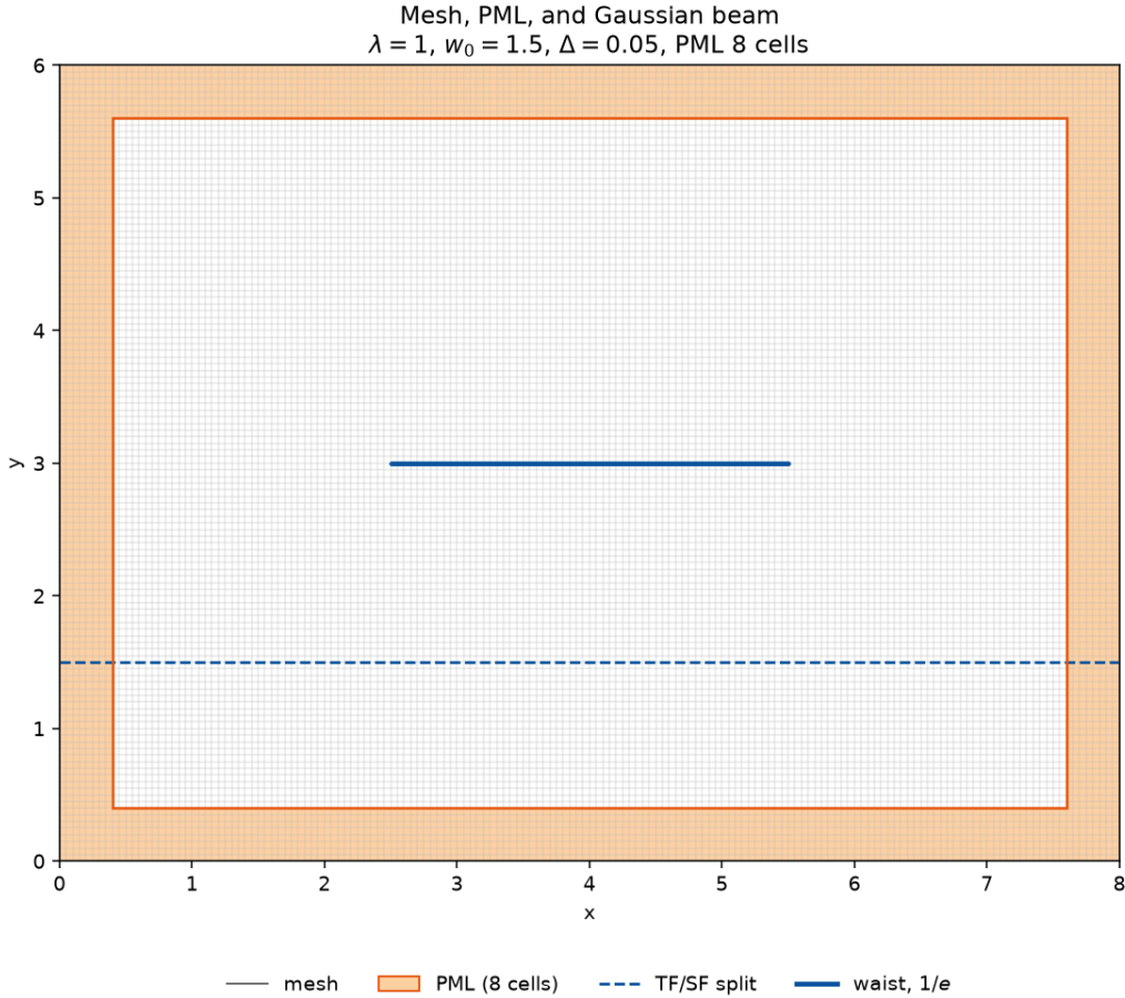
Figure 17: Default Gaussian-beam domain. The orange frame is the PML band used by the solve. The dashed line is the total-field/scattered-field split. The solid segment is the 1/e waist.
