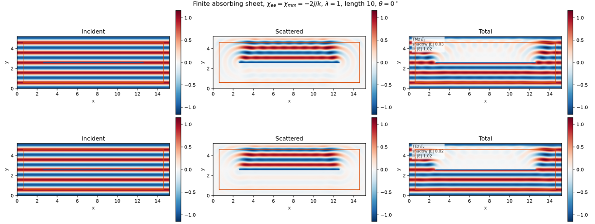
Figure 24: Finite absorbing sheet, \chi_{ee} = \chi_{mm} = -2j/k , \lambda = 1 , length 10\lambda , \theta = 0^\circ , at 20 cells per wavelength with 12 PML cells on each side. The rows are \text{Re } E_z (TMz) and \text{Re } E_x (TEz). The columns are the incident wave, the scattered field, and the total field. The annotated means are the lit side and the shadow over the central 6\lambda of the sheet.
