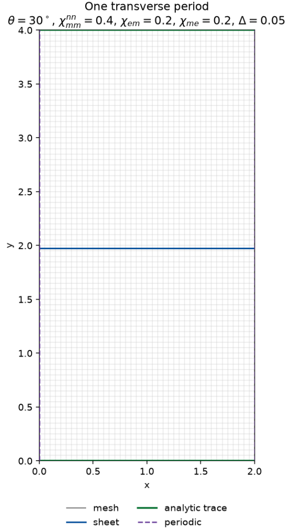
Figure 28: Periodic magneto-electric domain. The blue line is the sheet on a magnetic face. The green lines are the analytic trace on the y ends. The dashed purple lines mark the periodic identification of the x ends. The susceptibilities add \chi_{em} = \chi_{me} = 0.2 to the tangential and normal values of Figure 24.
