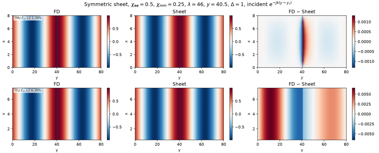
Figure 20: Symmetric sheet at \chi_{ee} = 0.5 , \chi_{mm} = 0.25 , \lambda = 46 , y = 40.5 , on an 8 \times 80 box at \Delta = 1 . The rows are \text{Re } E_z (TMz) and \text{Re } E_x (TEz). The annotated L^2 is the packed free electric vector.
