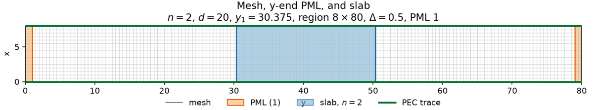
Figure 3: Default Fresnel domain. Orange bands are the y -end PML thickness drawn on the figure. Green edges are the PEC trace at x = 0 and x = 8 .
