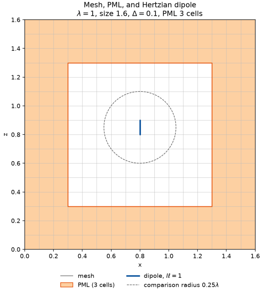
Figure 15: Default Hertzian-dipole domain. The orange frame is the PML band used by the solve. The blue segment is the z -directed element. The dashed circle is the 0.25\lambda radius inside which the field comparison is omitted.
