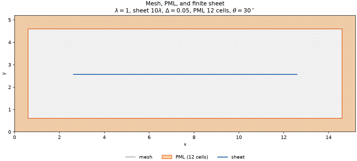
Figure 26: Finite oblique-sheet domain. The blue segment is the 10\lambda sheet on a magnetic face. The orange frame is the PML band on all four sides. The incidence is 30^\circ and the susceptibilities are \chi_{ee} = 0.5 , \chi_{mm} = 0.25 , \chi_{mm}^{nn} = 0.4 .
