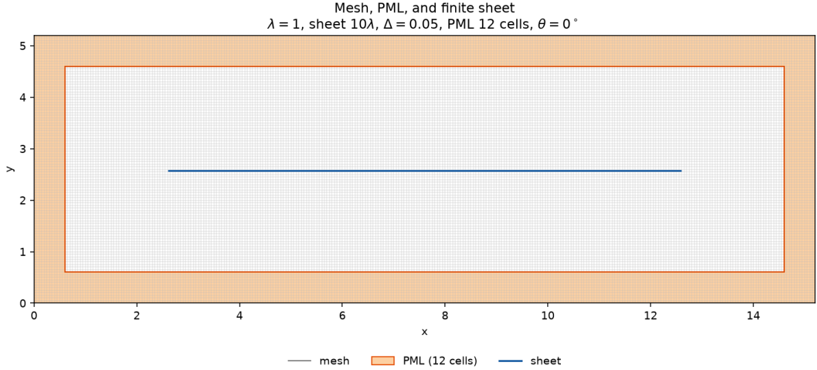
Figure 21: Default finite-sheet domain. The blue segment is the 10\lambda sheet on a magnetic face. The orange frame is the PML band on all four sides. The wall behind that band is PEC.
