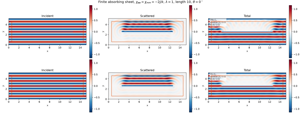
Figure 22: Finite absorbing sheet, \chi_{ee} = \chi_{mm} = -2j/k , \lambda = 1 , length 10\lambda , \theta = 0^\circ , at 20 cells per wavelength with 12 PML cells on each side. The rows are \text{Re } E_z (TMz) and \text{Re } E_x (TEz). The columns are the incident wave, the scattered field, and the total field. The annotated means are the lit side and the shadow over the central 6\lambda of the sheet.
