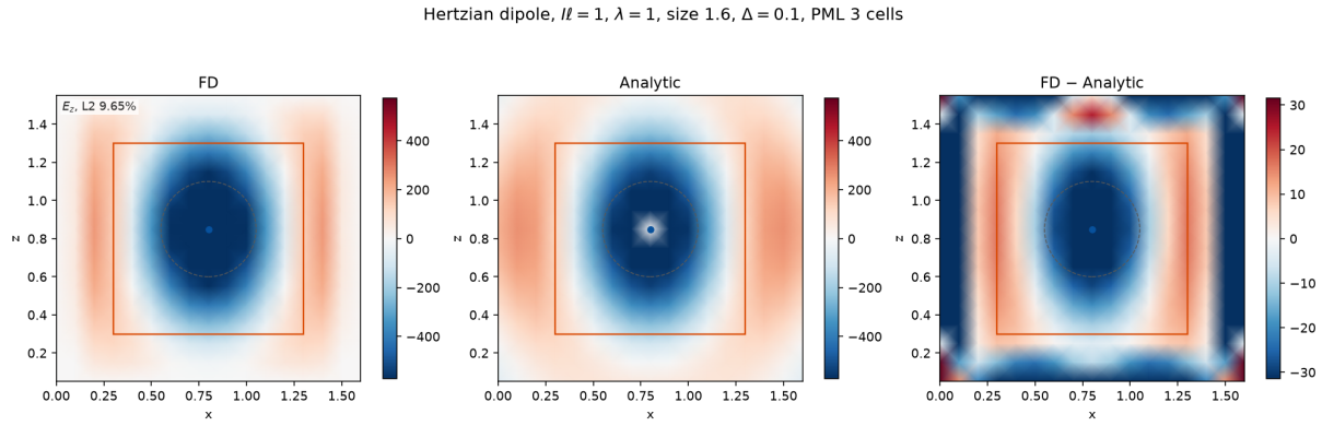
Figure 16: Hertzian dipole of moment I\ell = 1 at \lambda = 1 , on a cube of side 1.6 at \Delta = 0.1 , with three PML cells on each face. The panels are \text{Re } E_z on the xz plane through the element. The annotated L^2 is the electric-sample error outside the PML and at least 0.25\lambda from the element.
