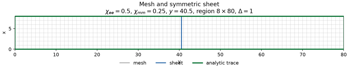
Figure 19: Default symmetric-sheet domain. The blue line is the sheet on a magnetic face. The green frame is the analytic trace on all four walls.
