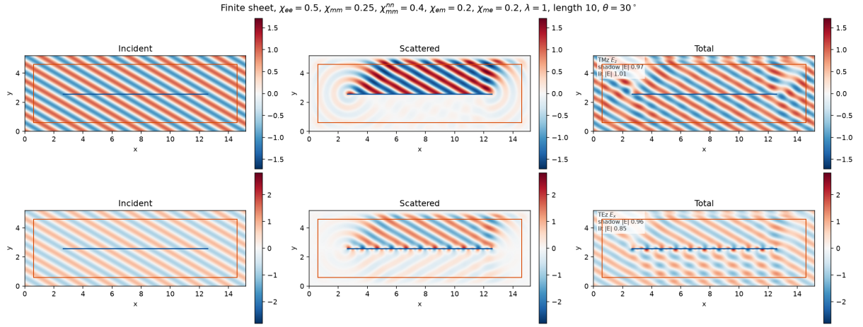
Figure 31: Finite sheet at \chi_{ee} = 0.5 , \chi_{mm} = 0.25 , \chi_{mm}^{nn} = 0.4 , \chi_{em} = \chi_{me} = 0.2 , \lambda = 1 , length 10\lambda , \theta = 30^\circ , at 20 cells per wavelength with 12 PML cells on each side. The rows are \text{Re } E_z (TMz) and \text{Re } E_x (TEz). The columns are the incident wave, the scattered field, and the total field. The annotated means are the lit side and the shadow over the central 6\lambda of the sheet.
