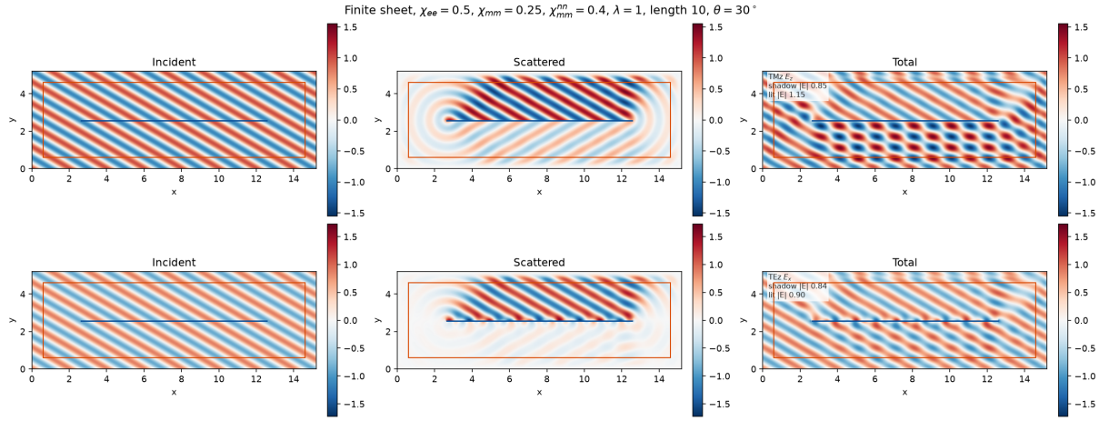
Figure 25: Finite sheet at \chi_{ee} = 0.5 , \chi_{mm} = 0.25 , \chi_{mm}^{nn} = 0.4 , \lambda = 1 , length 10\lambda , \theta = 30^\circ , at 20 cells per wavelength with 12 PML cells on each side. The rows are \text{Re } E_z (TMz) and \text{Re } E_x (TEz). The columns are the incident wave, the scattered field, and the total field. The annotated means are the lit side and the shadow over the central 6\lambda of the sheet.
