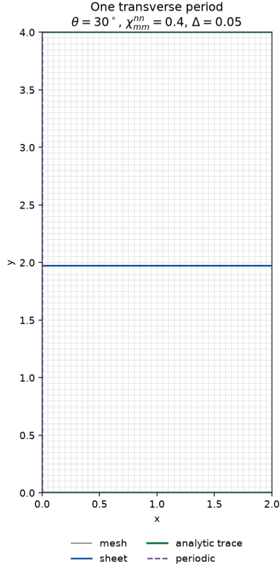
Figure 22: Default periodic-sheet domain. The blue line is the sheet on a magnetic face. The green lines are the analytic trace on the y ends. The dashed purple lines mark the periodic identification of the x ends. The width is one transverse period at 30^\circ .
