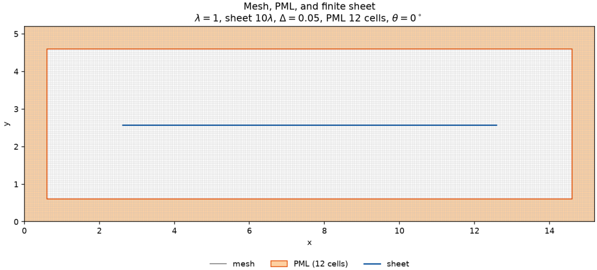
Figure 19: Default finite-sheet domain. The blue segment is the 10\lambda sheet on a magnetic face. The orange frame is the PML band on all four sides. The wall behind that band is PEC.
