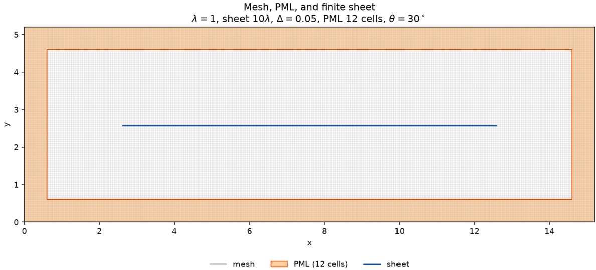
Figure 24: Finite oblique-sheet domain. The blue segment is the 10\lambda sheet on a magnetic face. The orange frame is the PML band on all four sides. The incidence is 30^\circ and the susceptibilities are \chi_{ee} = 0.5 , \chi_{mm} = 0.25 , \chi_{mm}^{nn} = 0.4 .
