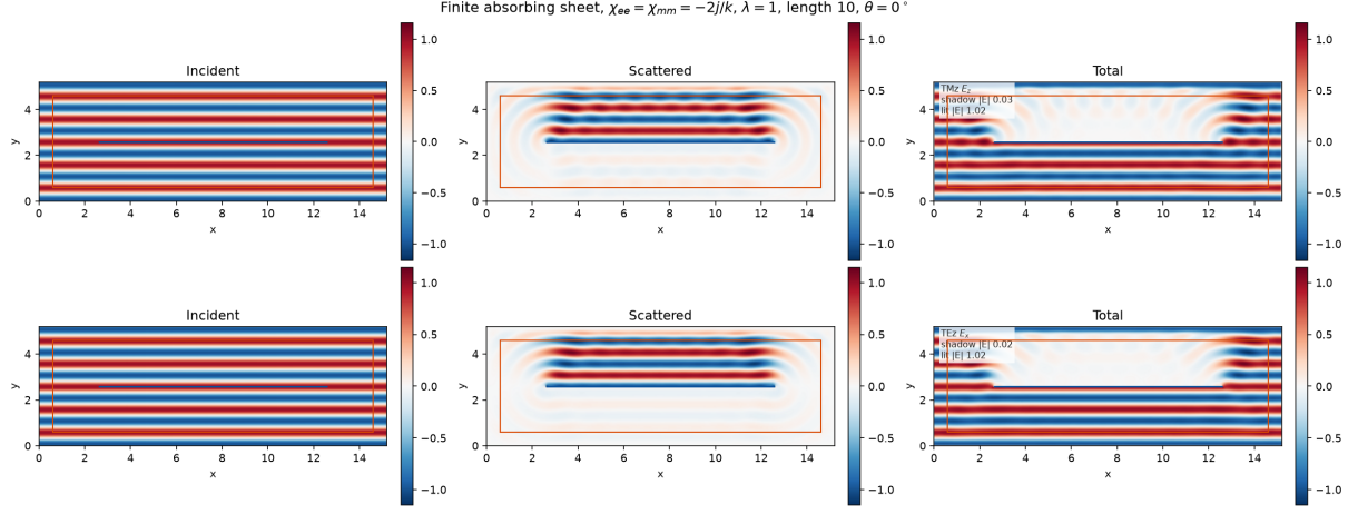
Figure 20: Finite absorbing sheet, \chi_{ee} = \chi_{mm} = -2j/k , \lambda = 1 , length 10\lambda , \theta = 0^\circ , at 20 cells per wavelength with 12 PML cells on each side. The rows are \text{Re } E_z (TMz) and \text{Re } E_x (TEz). The columns are the incident wave, the scattered field, and the total field. The annotated means are the lit side and the shadow over the central 6\lambda of the sheet.
