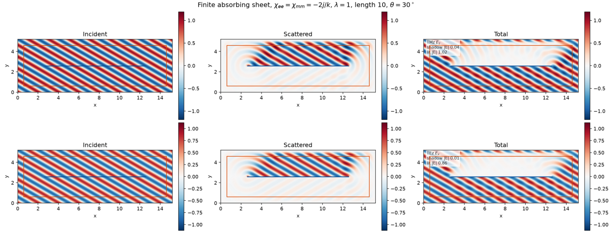
Figure 21: Finite absorbing sheet at \theta = 30^\circ , with \chi_{ee} = \chi_{mm} = -2j/k , \lambda = 1 , and length 10\lambda . The rows are \text{Re } E_z (TMz) and \text{Re } E_x (TEz). The annotated means are the lit side and the shadow over the central 6\lambda of the sheet.
