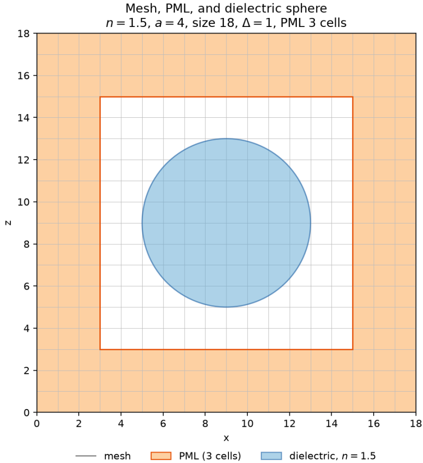
Figure 11: Default open-sphere domain. The orange frame is the PML band used by the solve. The disk is the cross-section of the staircase ball, n = 1.5 .
