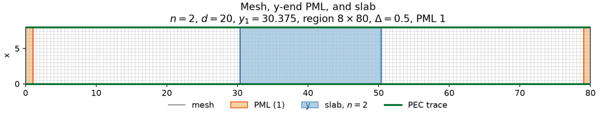
Figure 1: Default Fresnel domain. Orange bands are the y -end PML thickness drawn on the figure. Green edges are the PEC trace at x = 0 and x = 8 .
