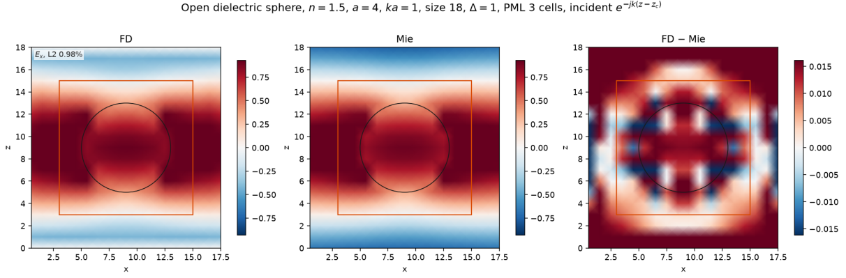
Figure 12: Open dielectric sphere at n = 1.5 , ka = 1 , a = 4 , on an 18^3 box at \Delta = 1 , with three PML cells on each face. The panels are \text{Re } E_x on the xz plane through the center. The annotated L^2 is the electric-sample error outside the PML and at least 2\Delta off the surface.
