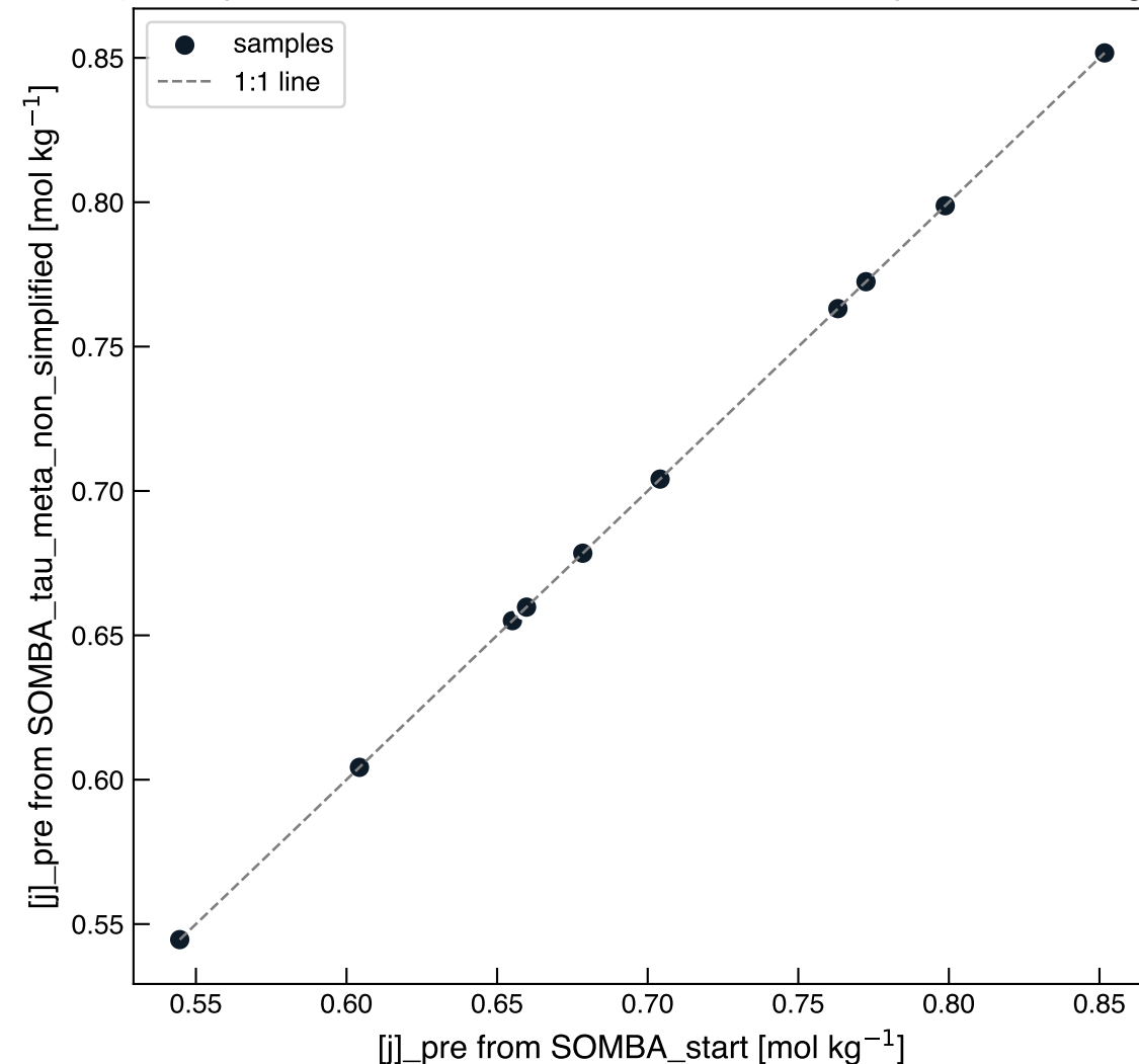
b) Comparison of calculated and reconstructed pre-weathering [j]
