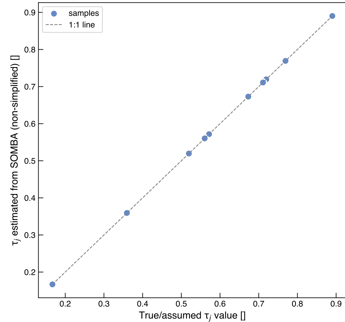
a) Comparison of assumed and estimated dissolution fractions
