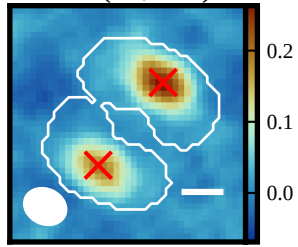
H 2 O(2 20 -2 11 )
