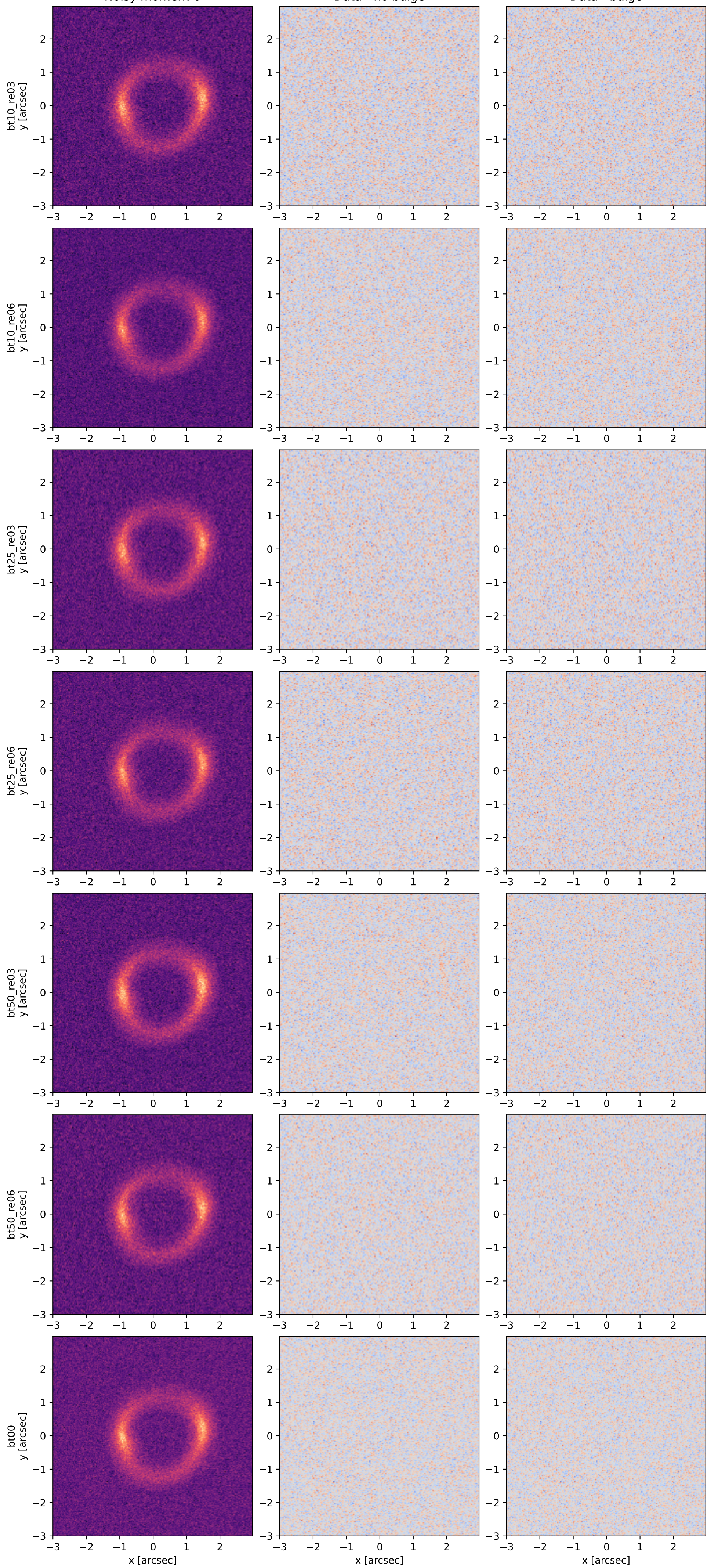
Noisy moment 0
