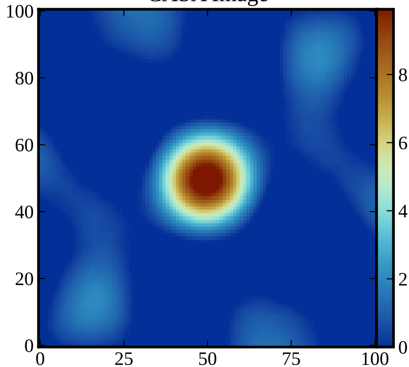
CASA Image
