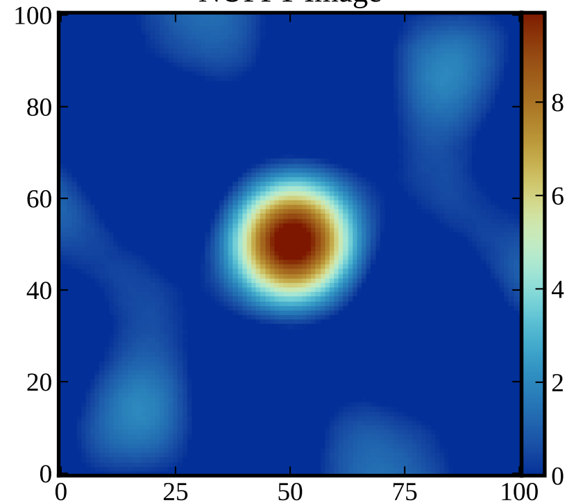
NUFFT Image
