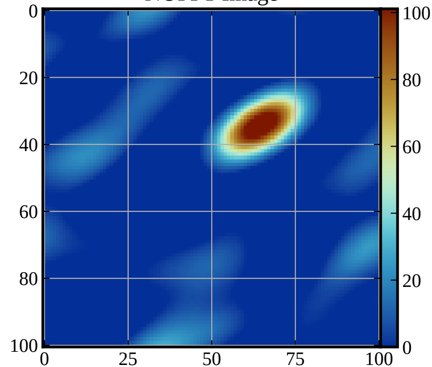
NUFFT Image
