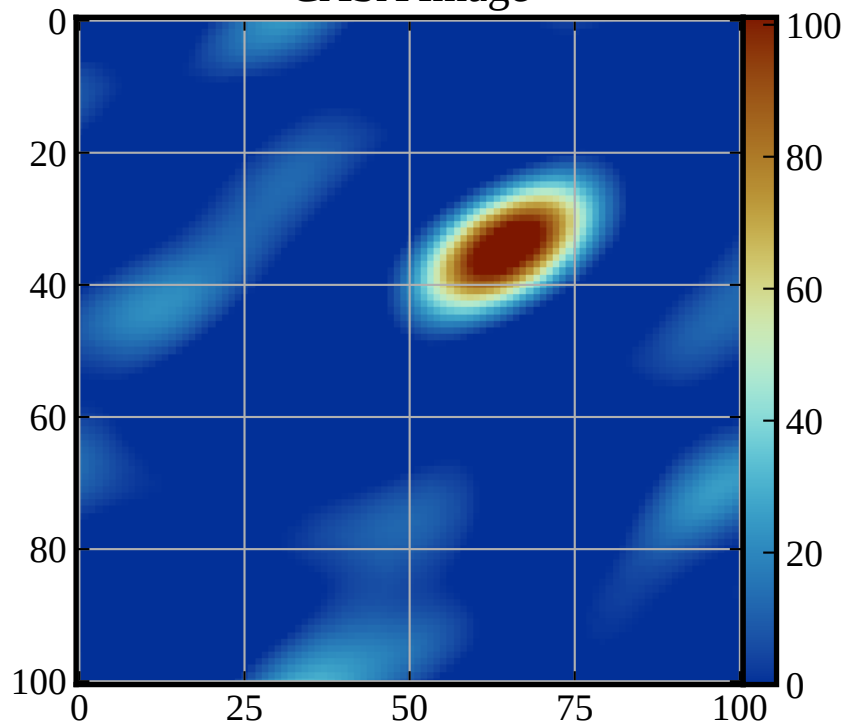
CASA Image
