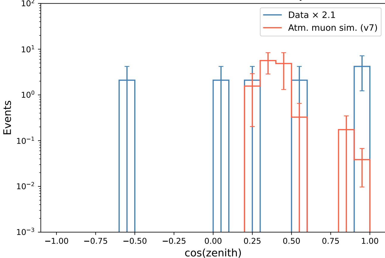
Zenith — >60 TeV (data \times 2.1 vs. v7 scaled by 63.56)
