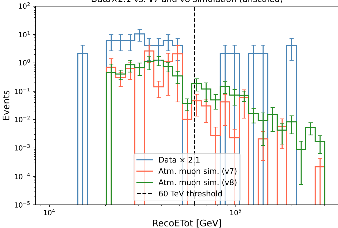
Data \times 2.1 vs. v7 and v8 simulation (unscaled)
