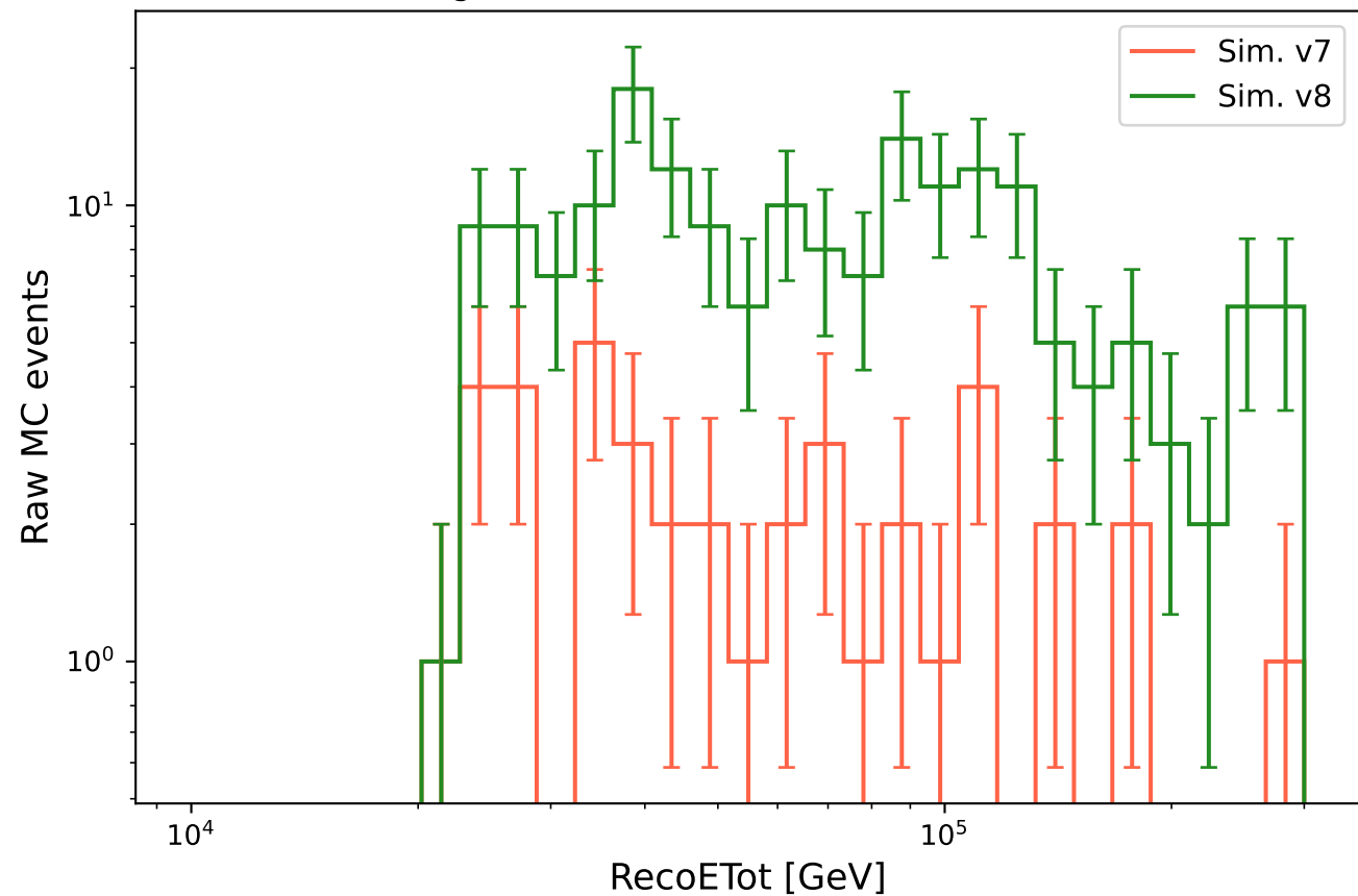
Unweighted simulated event counts — v7 vs v8
