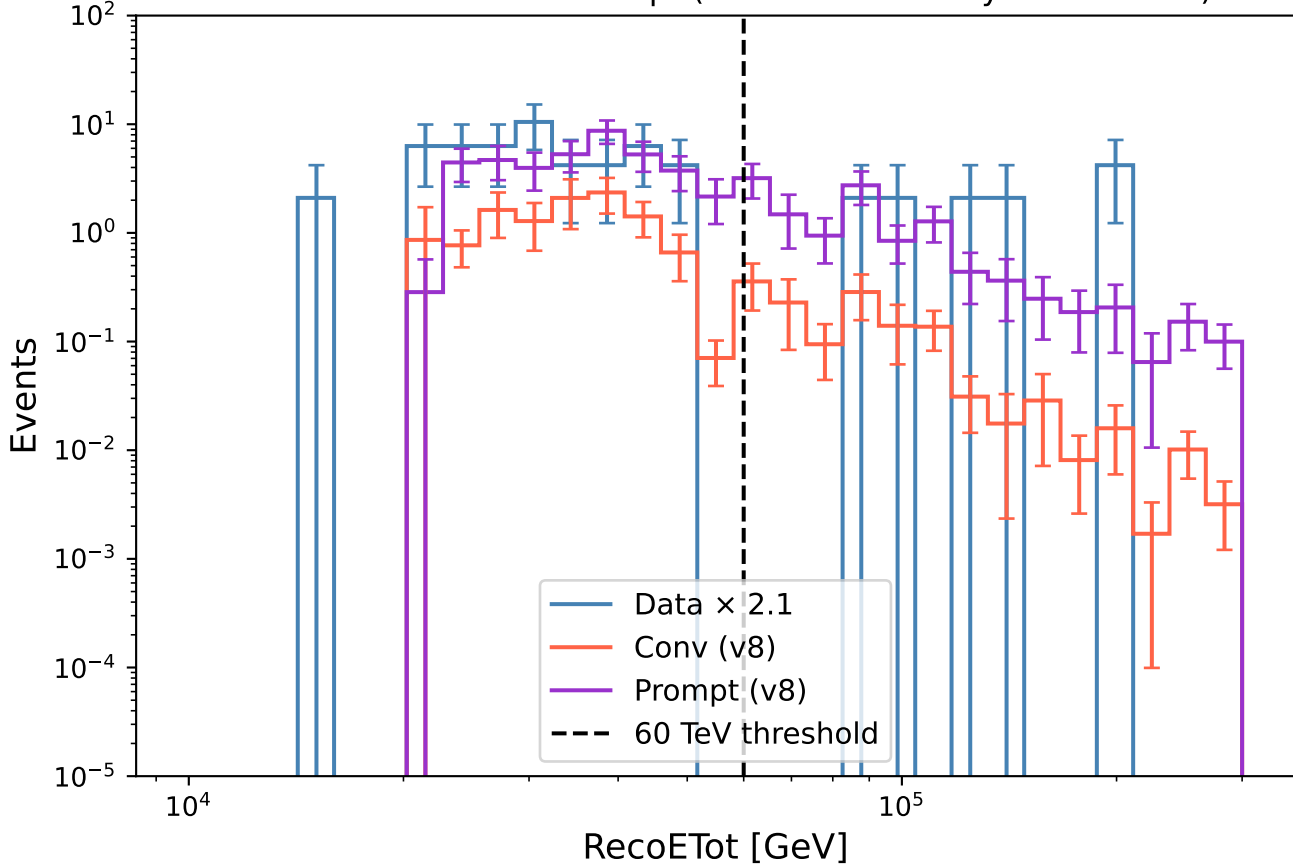
Data \times 2.1 vs. Conv + Prompt ( >60 TeV scaled by 1.89 \pm 0.82 )
