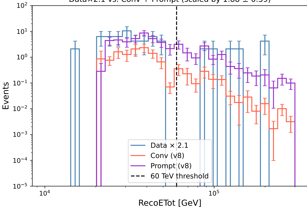
Data \times 2.1 vs. Conv + Prompt (scaled by 1.88 \pm 0.39 )
