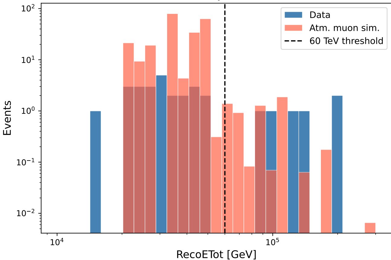
Data vs. simulation (scaled by >60 TeV ratio 30.3 \pm 16.8 )
