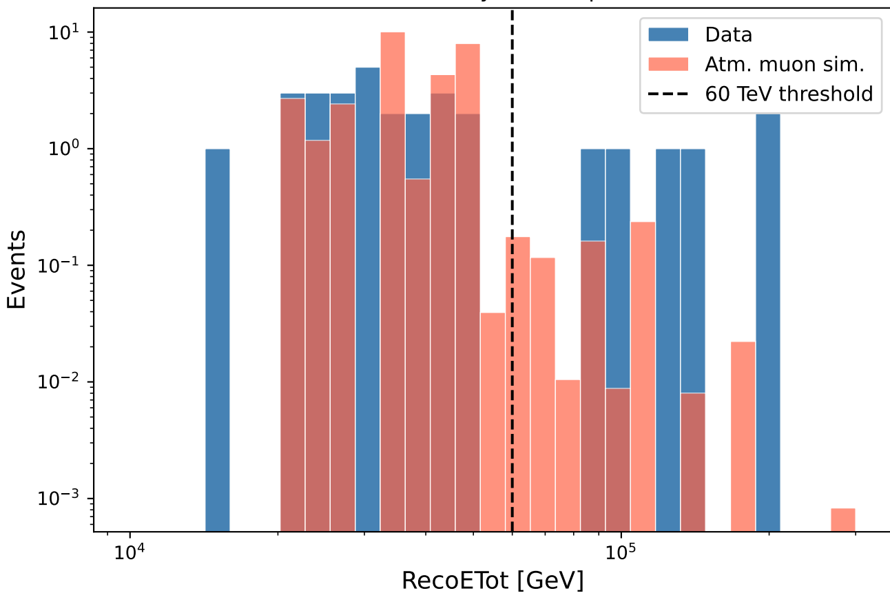
Data vs. simulation (scaled by full-sample ratio 3.82 \pm 1.59 )
