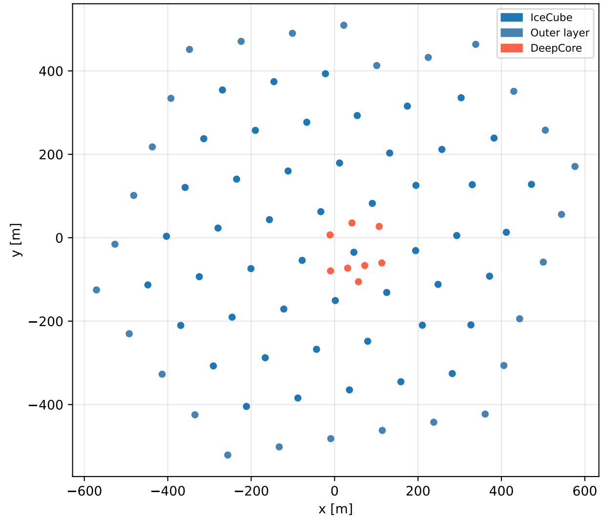
Top view (XY)
