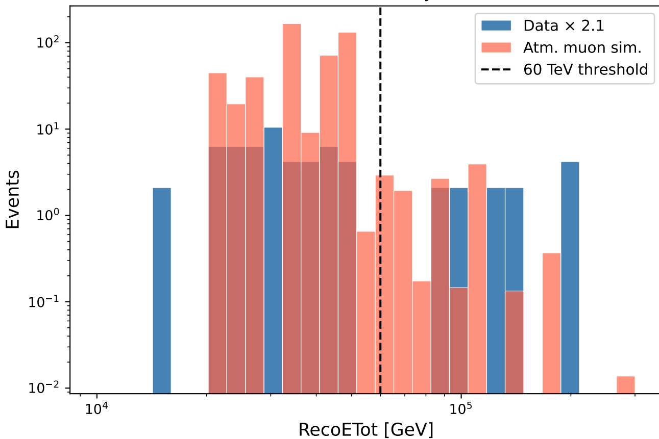
Data \times 2.1 vs. simulation (sim scaled by >60 TeV: 63.6 \pm 35.2 )
