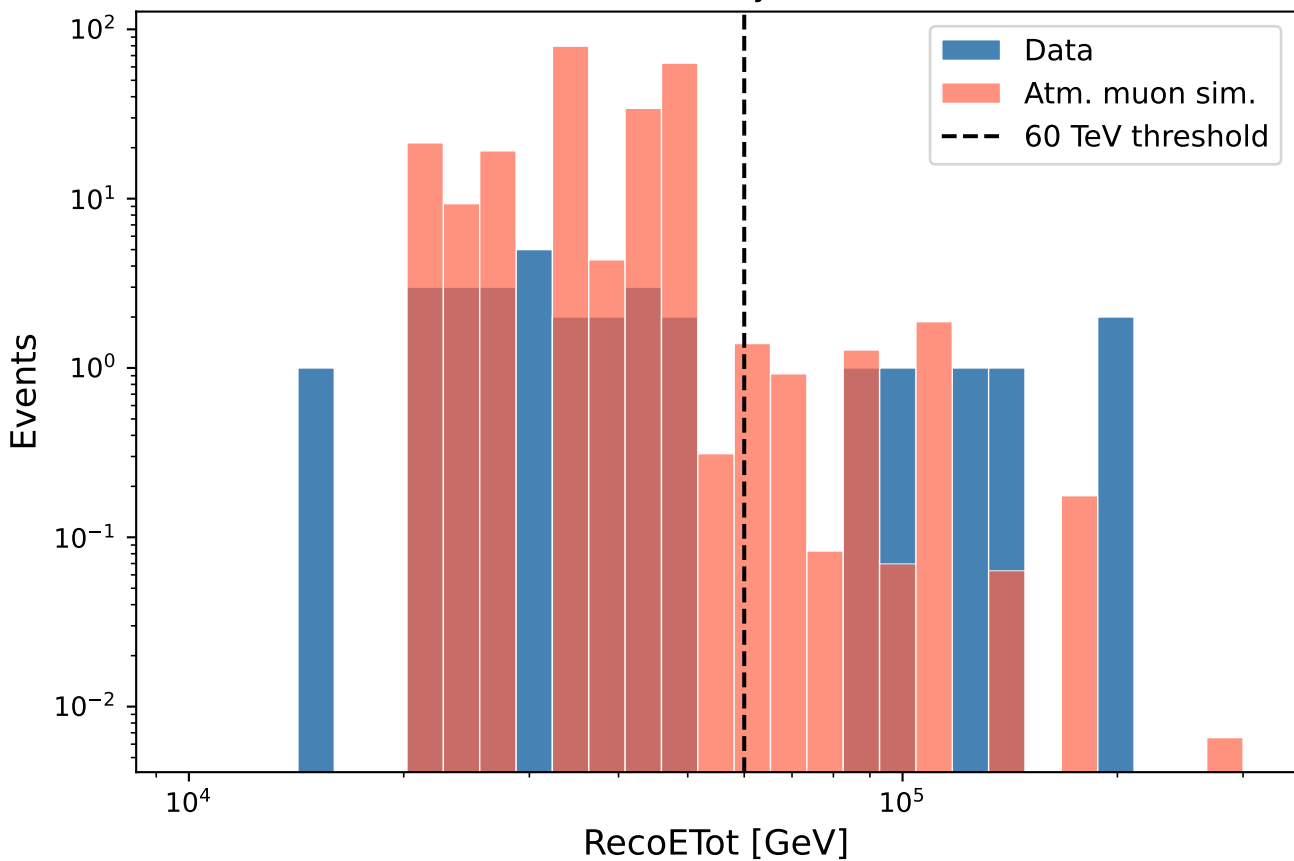
Data vs. simulation (sim scaled by >60 TeV ratio 30.3 \pm 16.8 )
